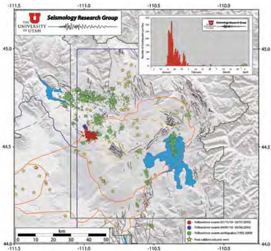
Figure 1. Map of Yellowstone National Park showing recent swarm earthquakes (red), previous swarms from 1995–2009 (green), volcanic vents (yellow stars), caldera boundaries (orange), Mallard Lake resurgent dome—to the southwest, and Sour Creek resurgent dome, to the northeast (yellow lines). Histogram shows the number of earthquakes per day from January 15 to April 6, 2010.
