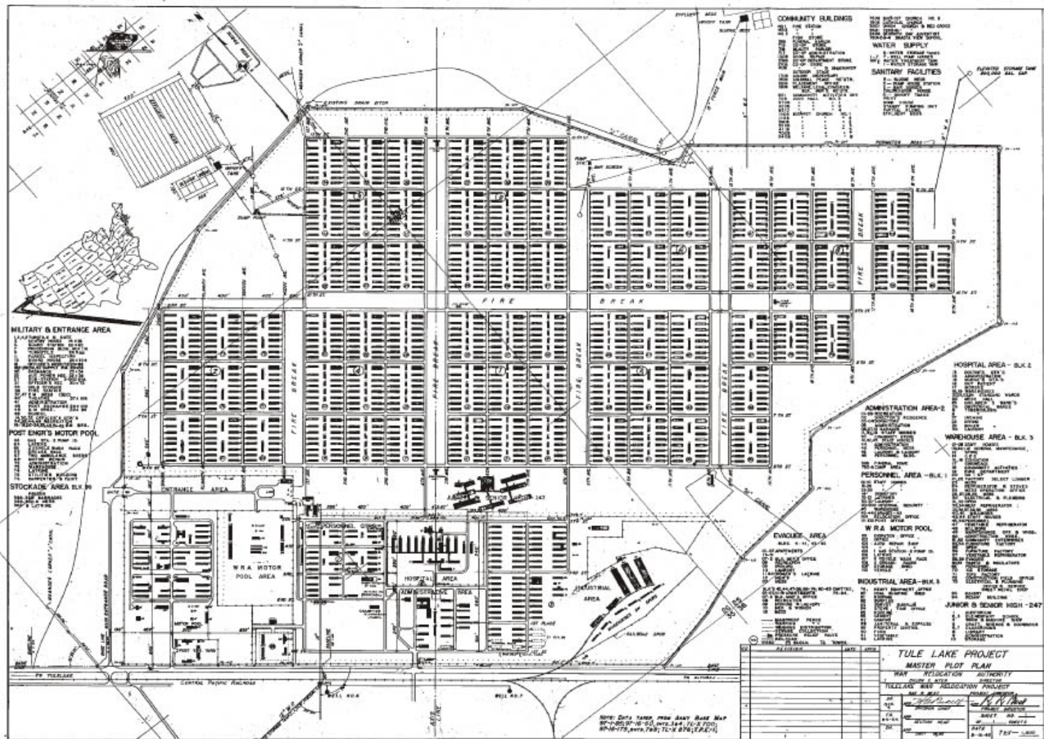
Figure 1 of 8. Tule Lake Master Plot Plan, August 1945.
