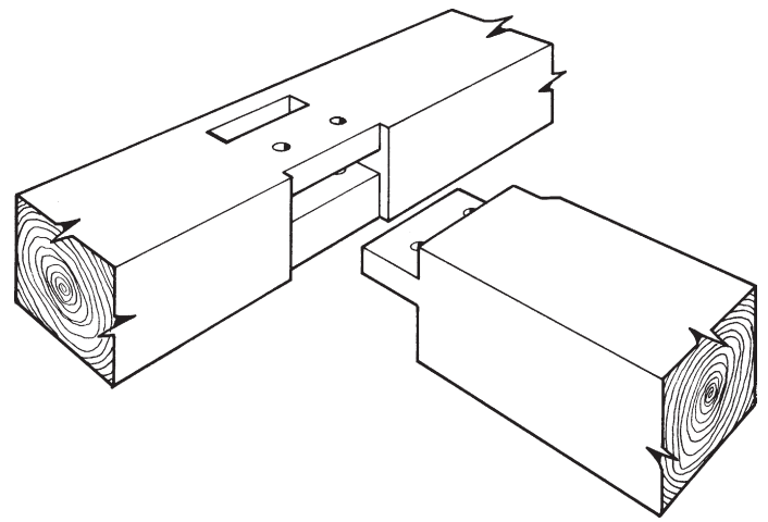
Fig. 4. Blind tenoned girder joint.
