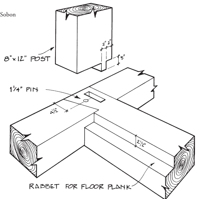
Fig. 6. Views of lapped half-dovetail girder joint in a pre-1820 scribe rule Dutch barn moved from Fort Plain to Altamont, N.Y. The interior sill is rabbetted for the 2 1/2-in. splined plank threshing floor.
