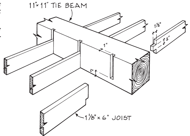
Fig. 27 (right). Board ceiling joists tenoned at one end and notched at the other drop into vertical chase mortises on the tie beams of the 1815 Methodist Church at Chenango Forks, New York (now dismantled). The bearing for the joist in the tie beam is only an inch deep. Close truss spacing of about 8 ft. permits the use of light boards. Similar joinery is found on an 1840 church in Brimfield, Massachusetts.
