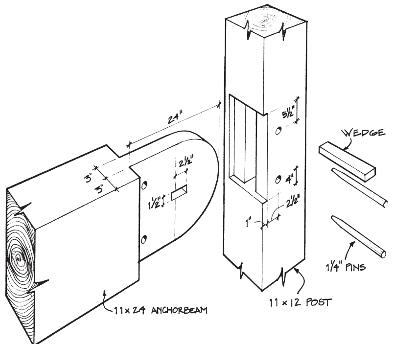
Fig. 14. Below, a through mortise and extended tenon as found in an 18th-century 47x45-ft. Dutch barn in Root, New York. Two pins and a single wedge secure this housed version. Note that the pins are not equidistant from the top and bottom of the tenon. Perhaps this was done to reduce the tendency of the 24-in.-deep white pine anchor beam to lift off the shoulder as it shrank.
