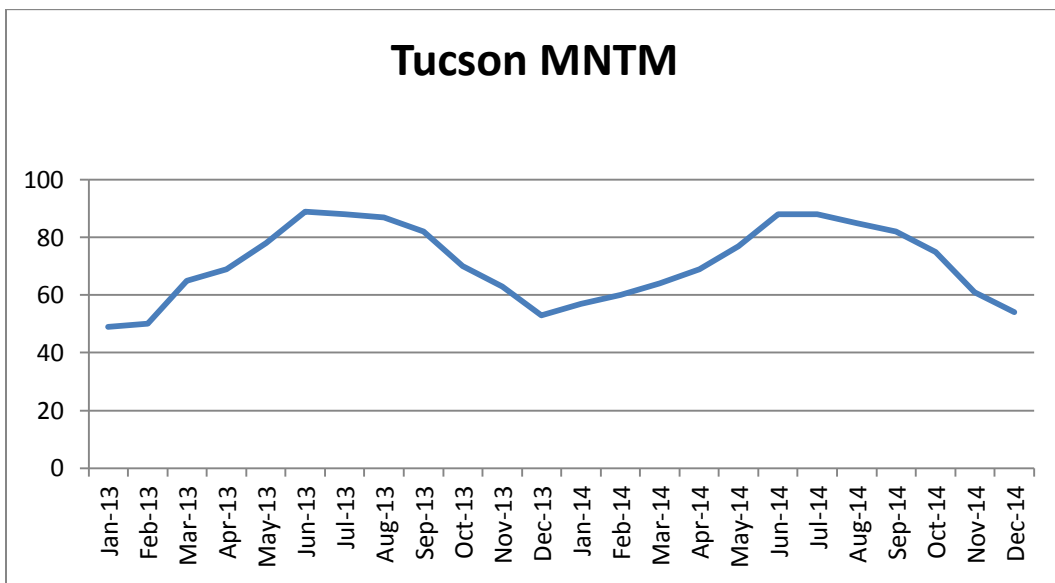
Figure 5. Mean monthly temperature 2013-2014.
