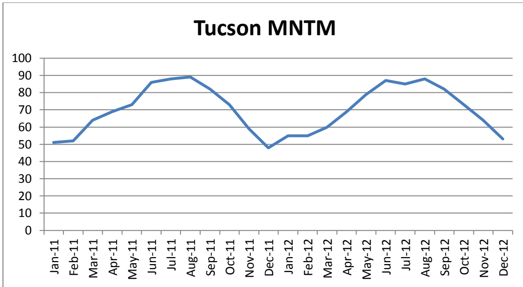
Figure 4. Mean monthly temperature 2011-2012.
