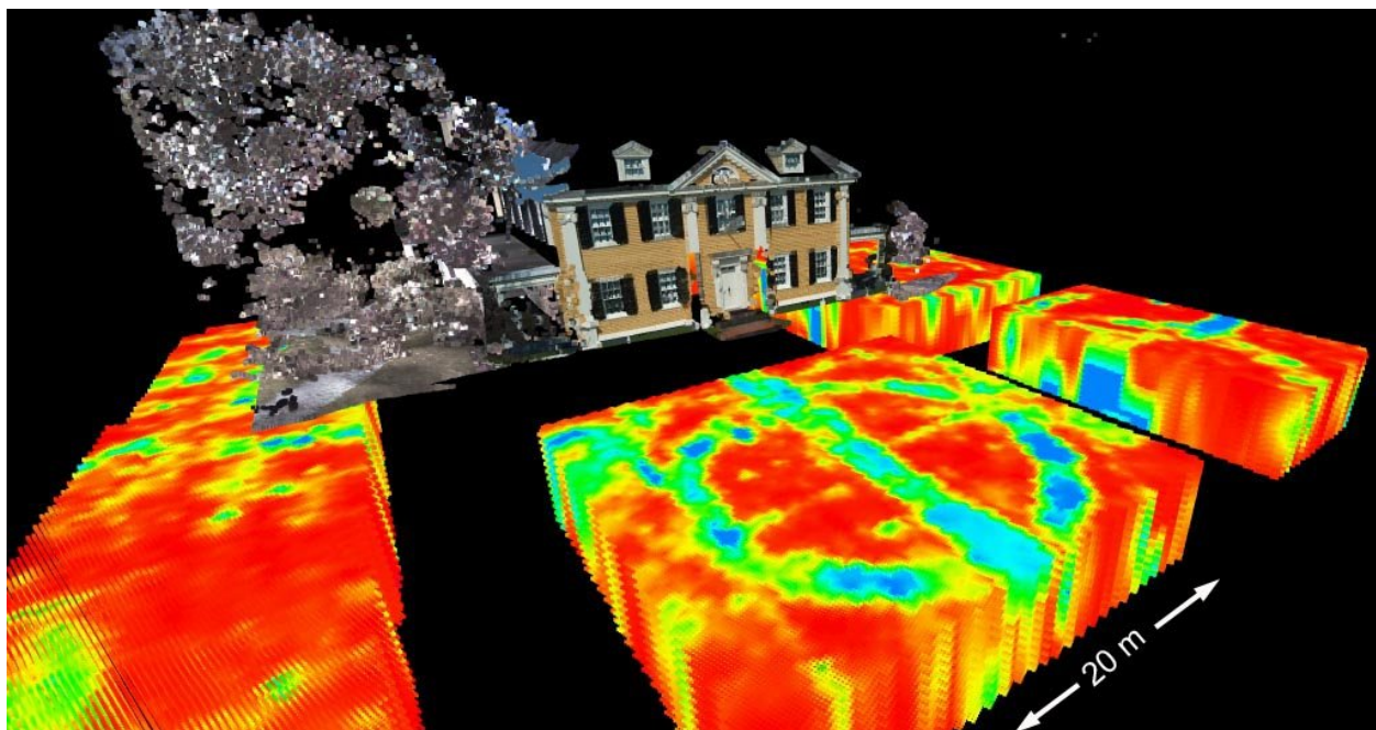
Figure 1 Laser scan and ground penetrating radar surveys of the Longfellow House - Washington's Headquarters NHS 3D model in Pointools.
