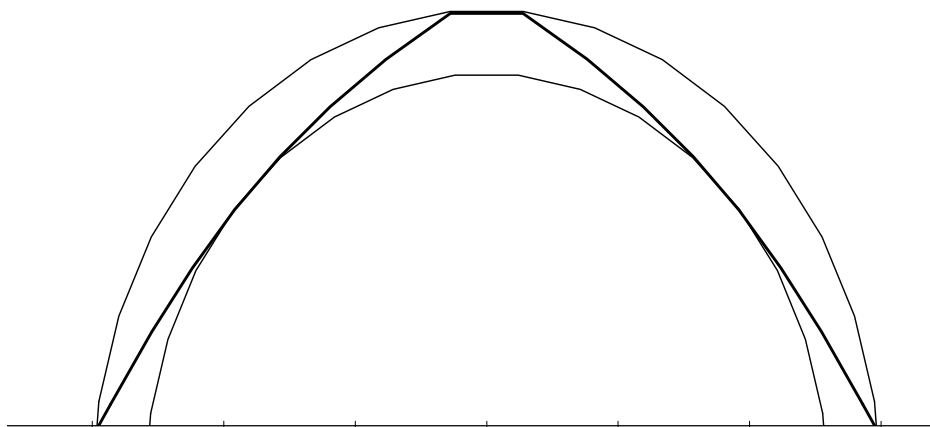
(d) self-weight + crown load: hinges at crown, supports, and haunches
