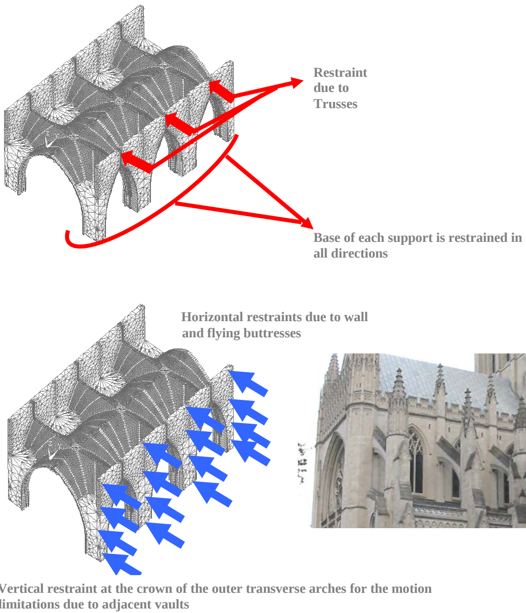
Figure 51: Final Boundary Conditions for the NC Triple-Vault Model
