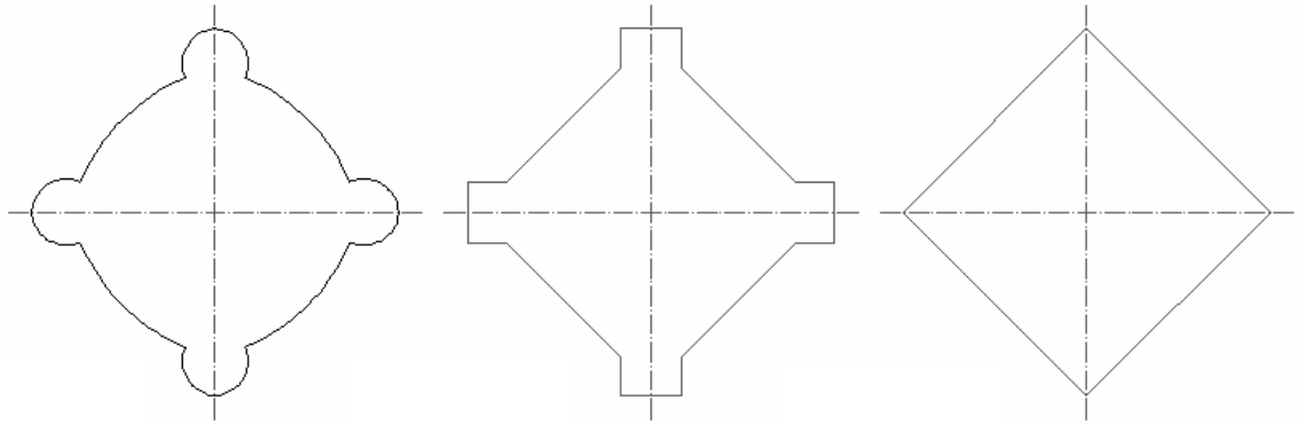
Figure 27: Geometric simplification of the center pier cross section with constant area.
