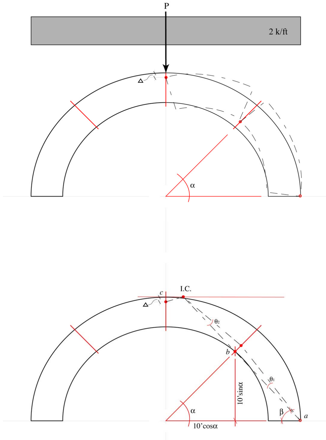
Figure 13: Collapse Mechanism for Crown Loading
