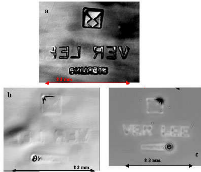
Figure 6. Three ultrasonic images of a sterling silver test coupon. (a) A 50 MHz F/2 back-wall image of the original hallmark. (b) A 50 MHz F/2 back-wall image of the residual deformation remaining in the coupon after the hallmark has been polished away. (c) A 20 MHz F/1 surface wave image of the same deformation in 6b except imaged from the surface containing the deformation
