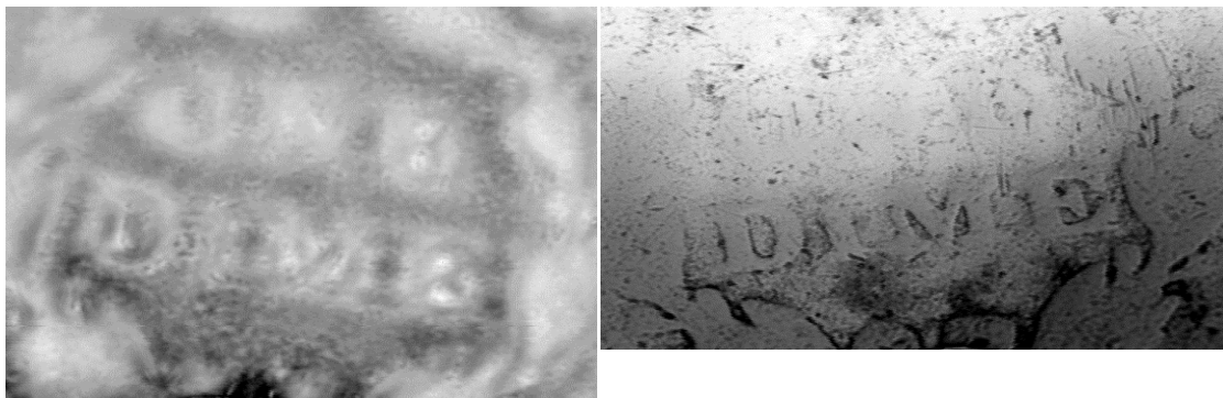
Figure 17. American silver dime dating from the 1840's. (A) Surface wave acoustic image made in FC-40 as the coupling medium. (B) Same image except water was used as the coupling medium for the direct reflection image
