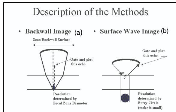
Figure 4. Schematic showing (a) back surface reflection imaging (or backwall imaging) and (b) mode converted surface wave imaging.
