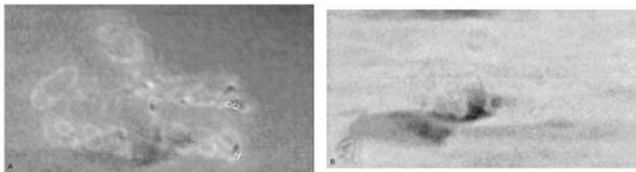
Figure 12. Effects of annealing on sterling silver. (A) A recovered acoustic image of polished-off hallmarks on a sterling silver coupon before annealing. (B) The same area after annealing the coupon.
