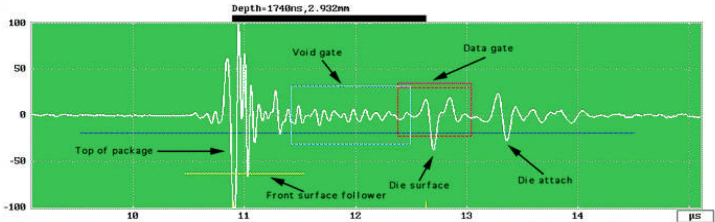
Figure 5. A typical acoustic pulse showing a ‘gate’ around that portion of the pulse to be processed to form an image. (source of image unknown)
