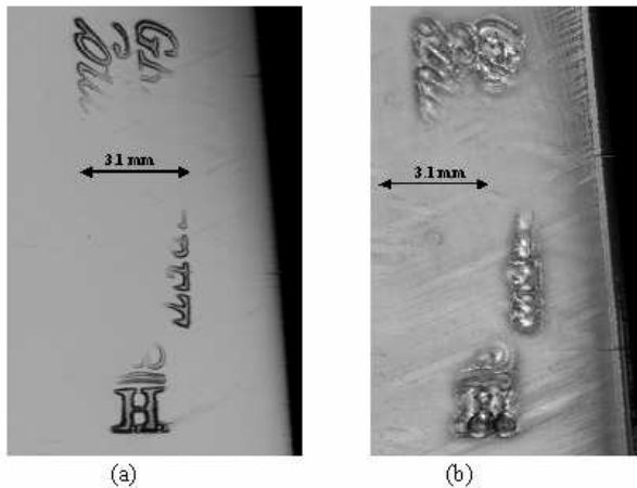
Figure 13. Silver dessert knife with a steel blade. (a) Direct reflection acoustic image. (b) Surface wave acoustic image of the same area.
