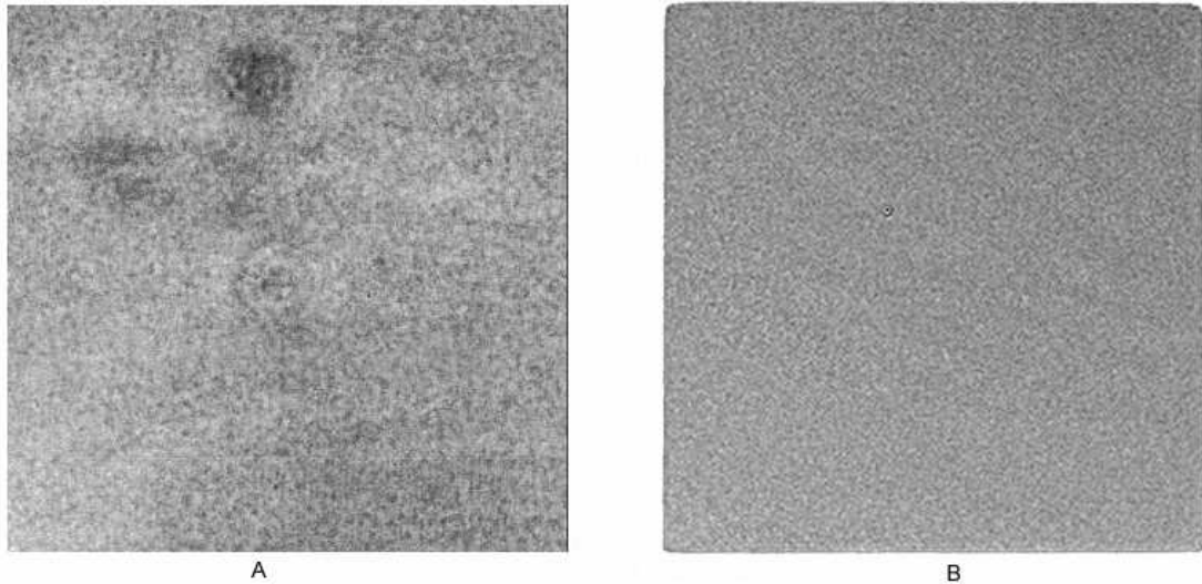
Figure 7. Acoustic images: (A) an 18K gold coupon and (B) a 22K gold coupon
