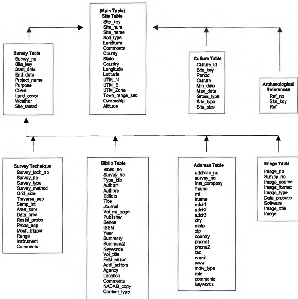
Figure 1. Organization of the NADAG database structure within Oracle 8 software.
