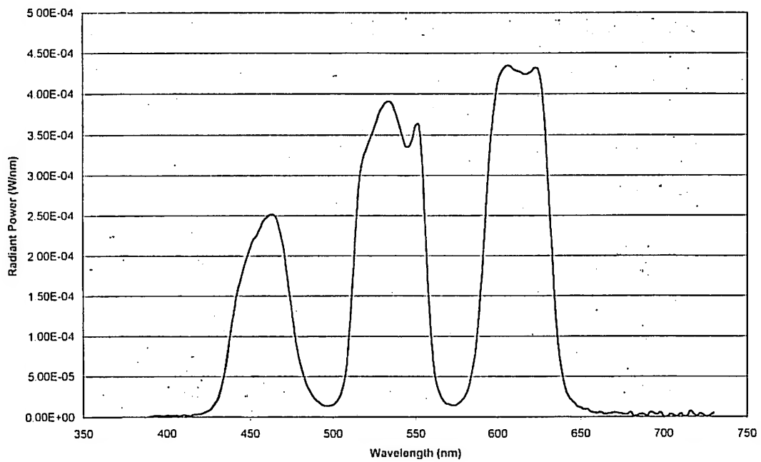
Figure 4 Spectral Power Distribution for 3-band source, 4200K
