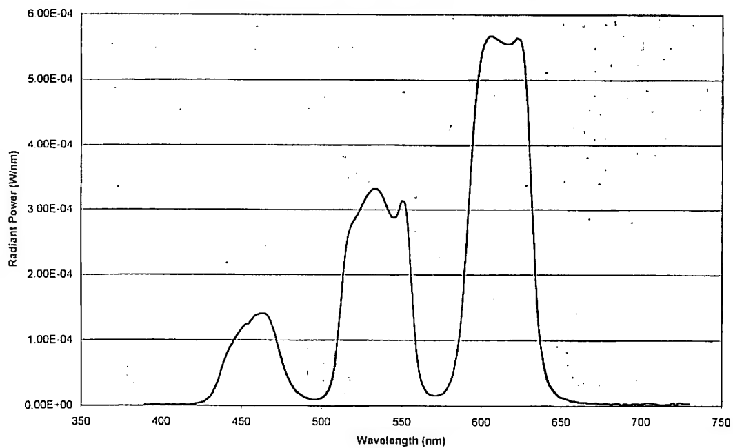
Figure 2 Spectral Power Distribution for 3-band source, 2850K
