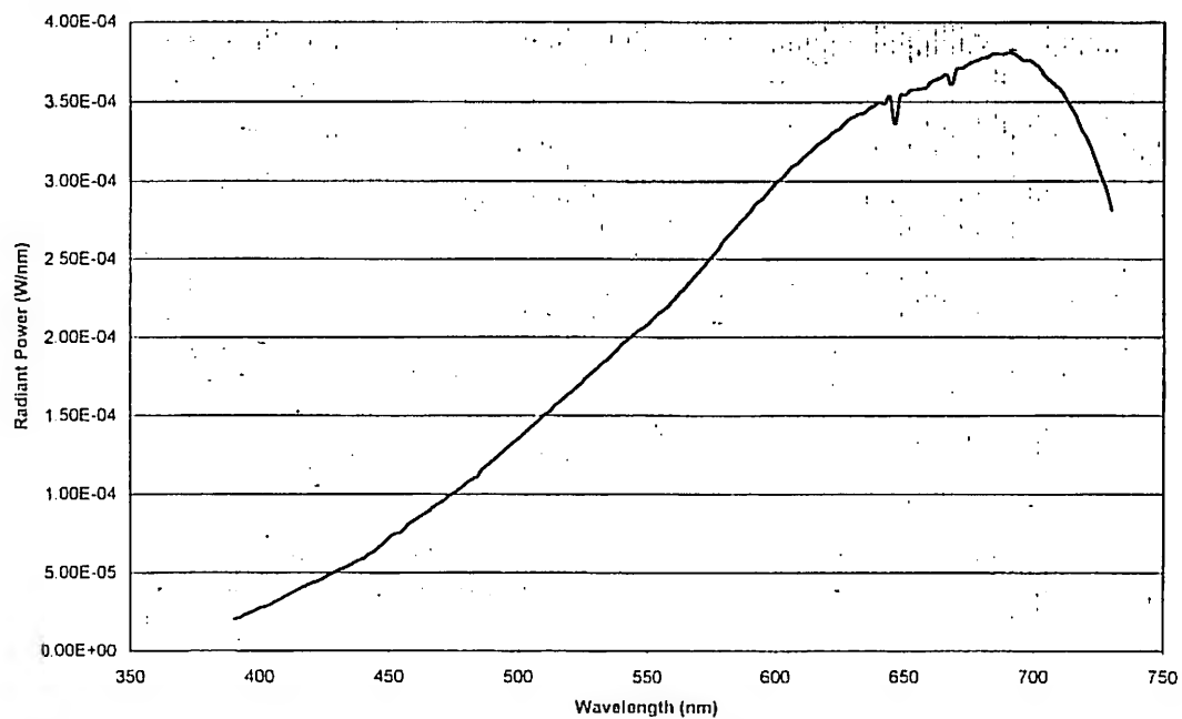
Figure 1 Spectral Power Distribution for MR lamp, 2850K
