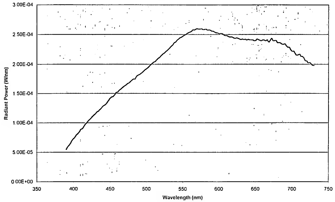
Figure 3 Spectral Power Distribution for MR lamp, 4200K
