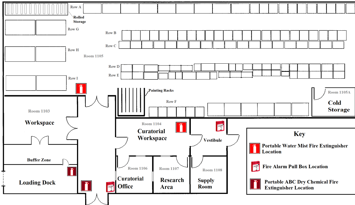
Portable Fire Extinguisher and Fire Alarm Pull Box Location Floor Plan: Curatorial Facility
