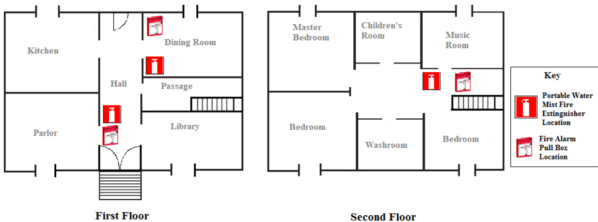
Portable Fire Extinguisher and Fire Alarm Pull Box Location Floor Plan: Hilltop House
