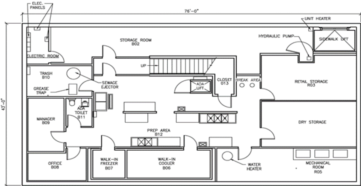
Lincoln Memorial North Basement Schematic
