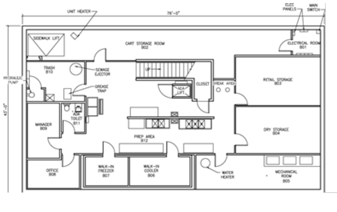
Lincoln Memorial South Schematic
