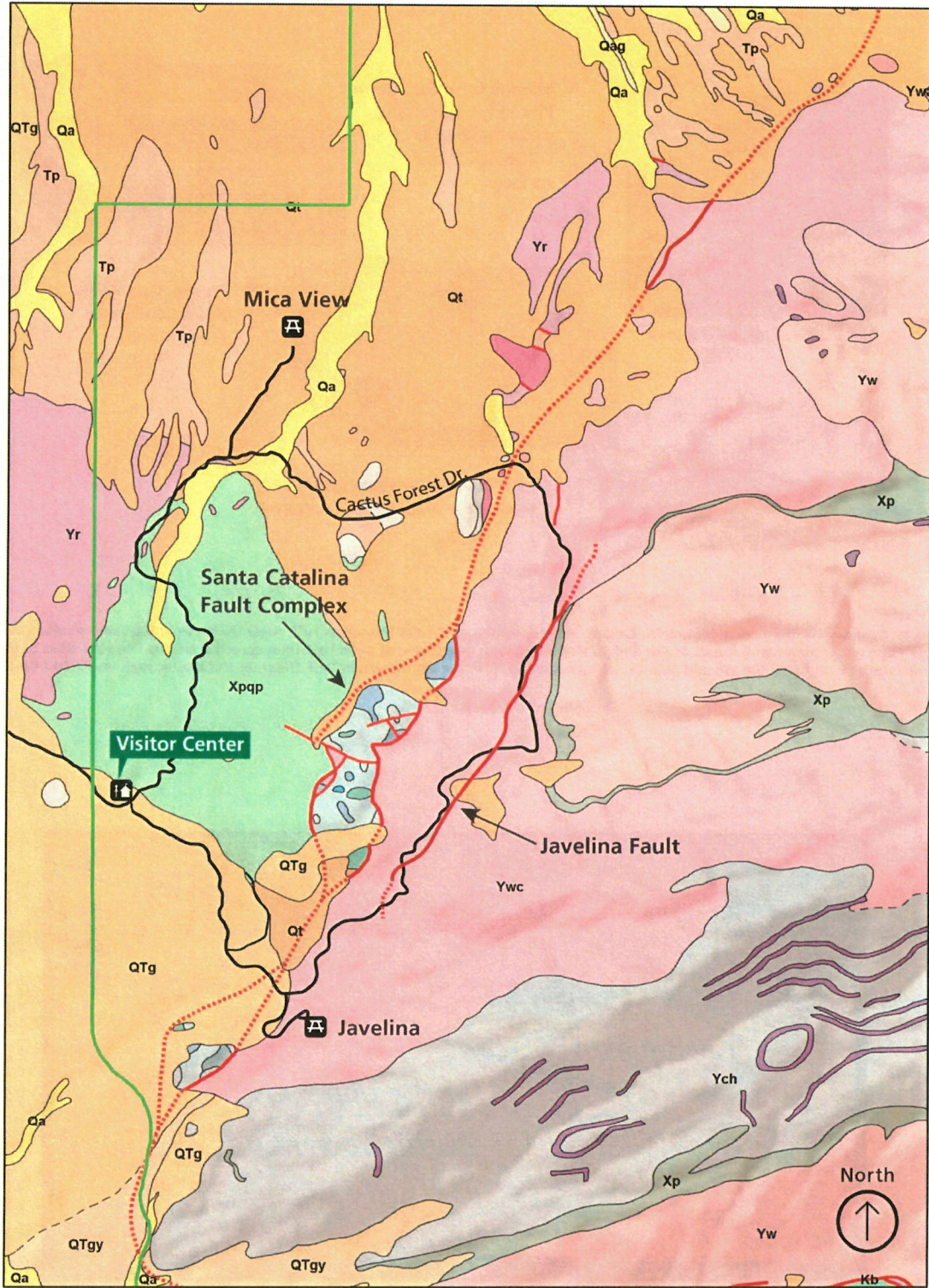
Figure 14. Location of the Javelina Fault in relation to the Santa Catalina Fault Complex, Rincon Mountain District, Saguaro National Park. Red lines represent the approximate location of each fault, dashed where not exposed on the surface. Geologic map unit symbols are described in the Map Unit Properties Table. Green line represents park boundary. Graphic by Phil Reiker (NPS Geologic Resources Division), compiled from GRI Digital Geologic Data of Saguaro National Park (Appendix A).
