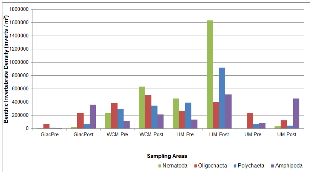
Figure 7. Density comparison of Nematoda (phylum), Oligochaeta (subclass), Polychaeta (class), and Amphipoda (class) between Study Areas.
