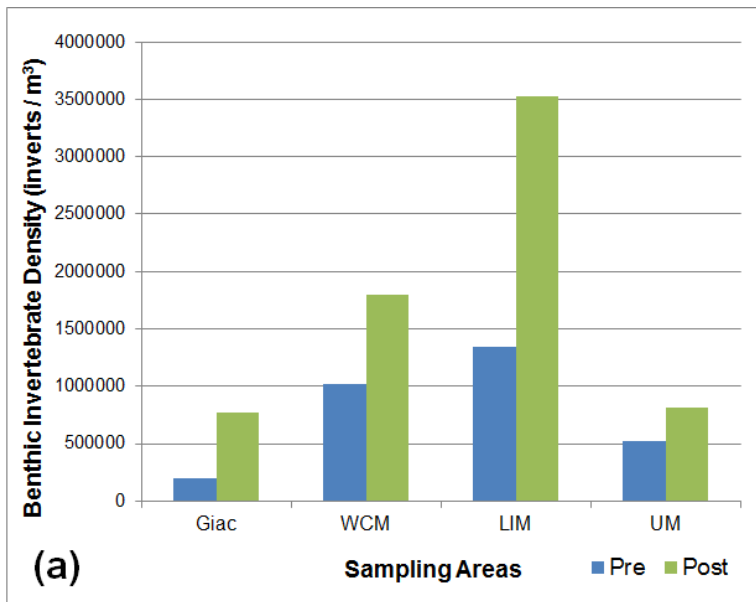
Figure 4. Histogram plot showing average total benthic invertebrate density at Giacomini Wetlands (Giac) and the three Reference Areas (WCM, LIM, and UM) pre- and post-restoration. Density is listed as number of invertebrates per m 3 of sediment.
