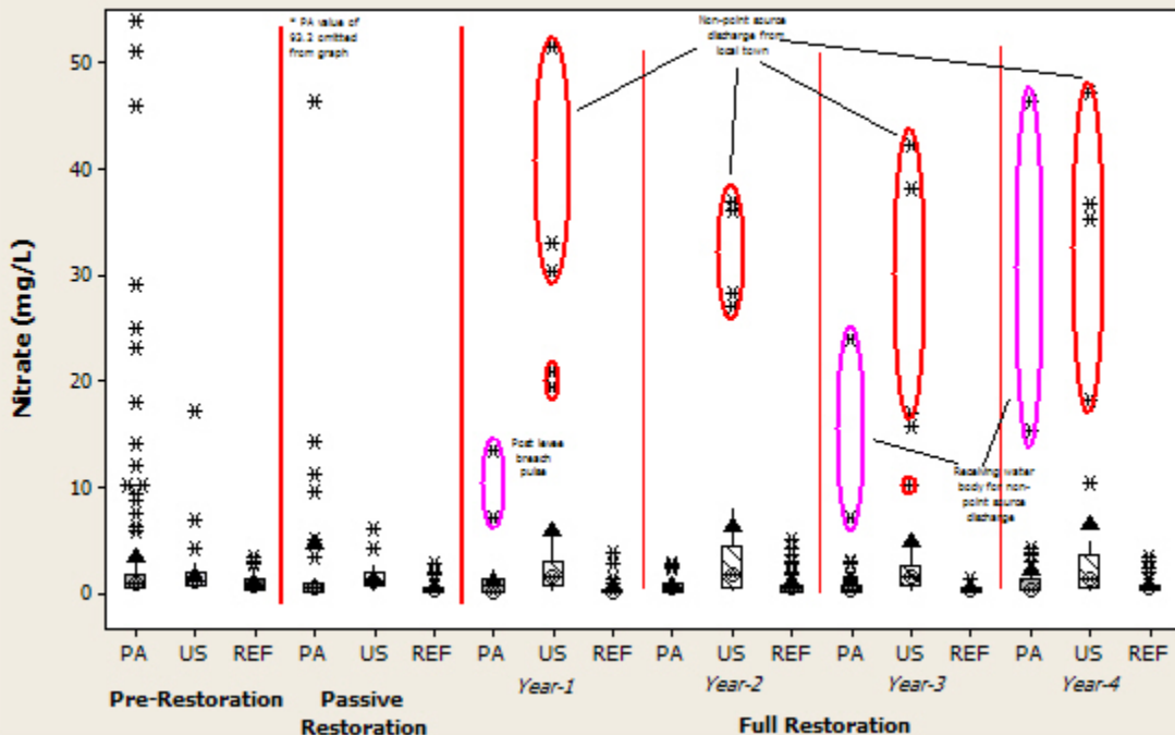
Figure 3. Average, median, and other summary statistics for nitrates ( \text{NO}_3^- ) for Study Areas Pre-Restoration, during Passive Restoration, and in the first four years of Full Restoration.
