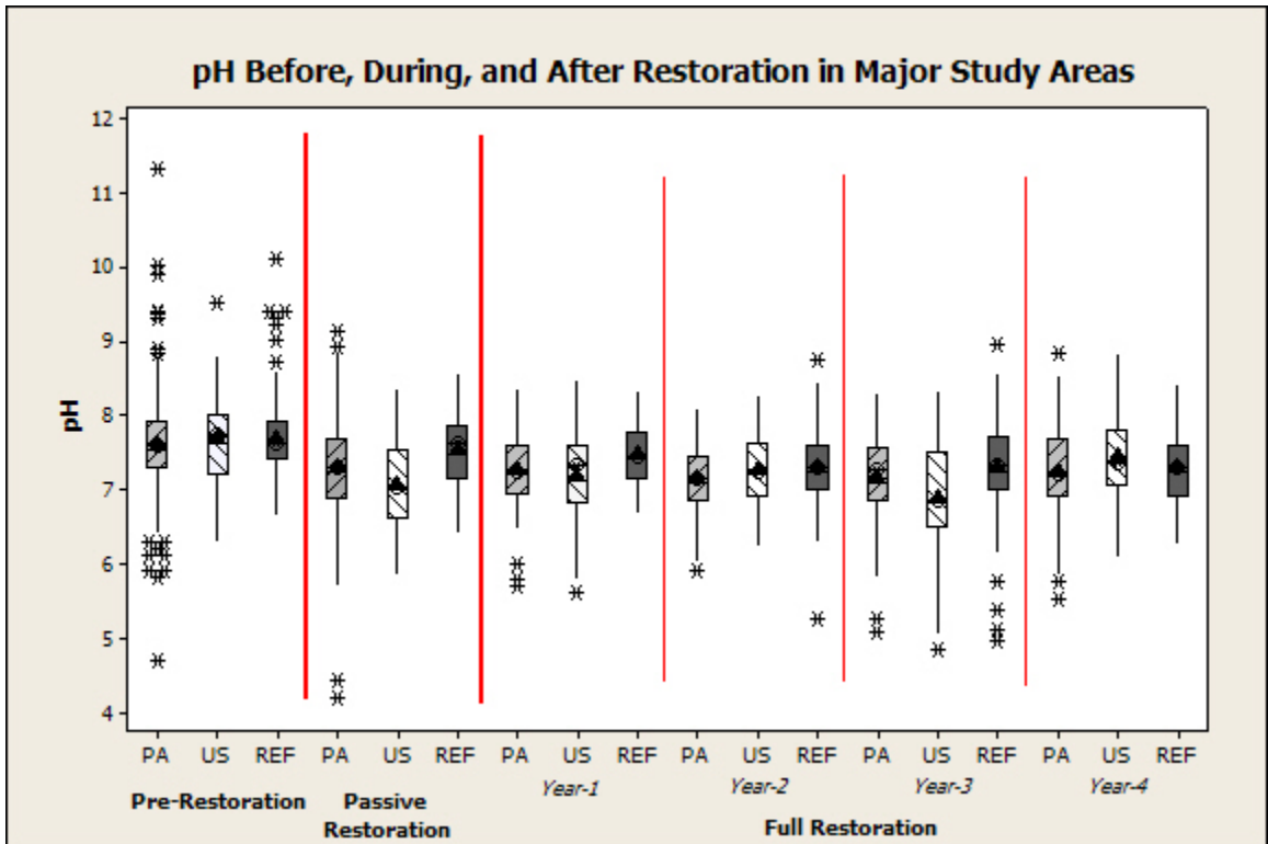
Figure 2. Average, median, and other summary statistics for pH for Study Areas Pre-Restoration, during Passive Restoration, and in the first four years of Full Restoration. Boxplots indicate first and third quartiles (25%, 75%). Lines indicate 10 th and 90 th percentiles. Medians are indicated by diagonal-hatched circle, with means designate by black triangles.
