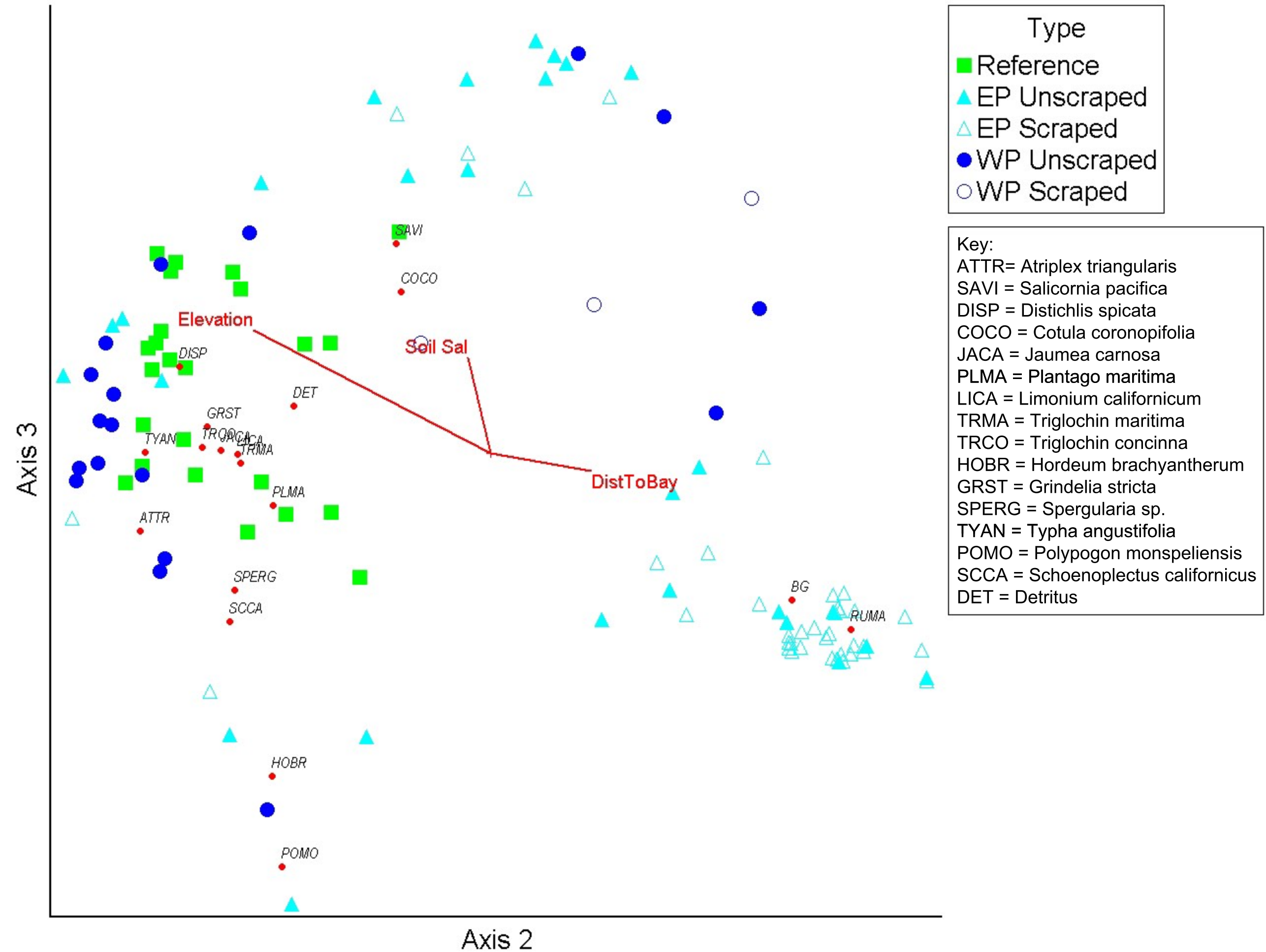
Figure A5. Axis 2 x Axis 3. NMS Results for 2011 Species Composition and Environmental Variables in the Restoration Project Area as compared to the Reference Sites. Final stress = 10.11246, Instability = 0.00603, Final dimensions = 3 (max = 6), 500 iterations. Axis 2 R^2 = 0.262 , Axis 3 R^2 = 0.440
