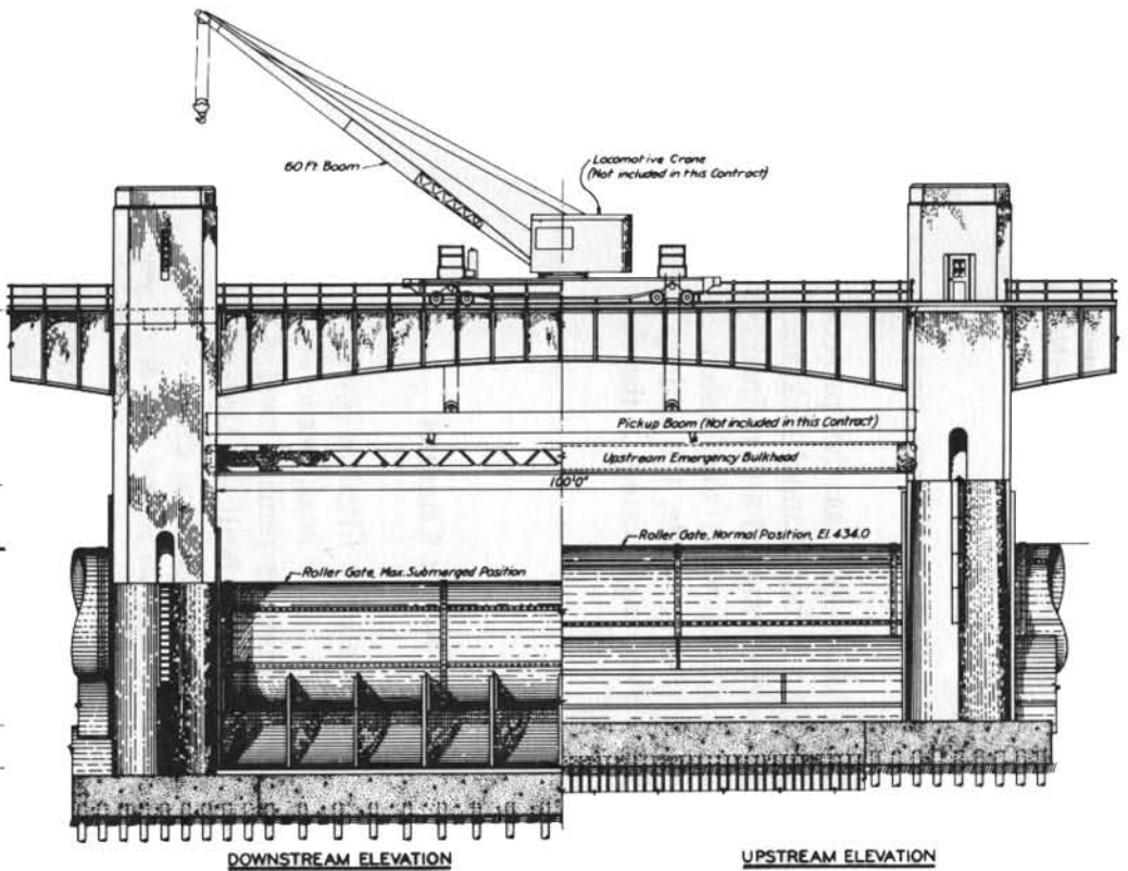
TYPICAL ELEVATIONS
