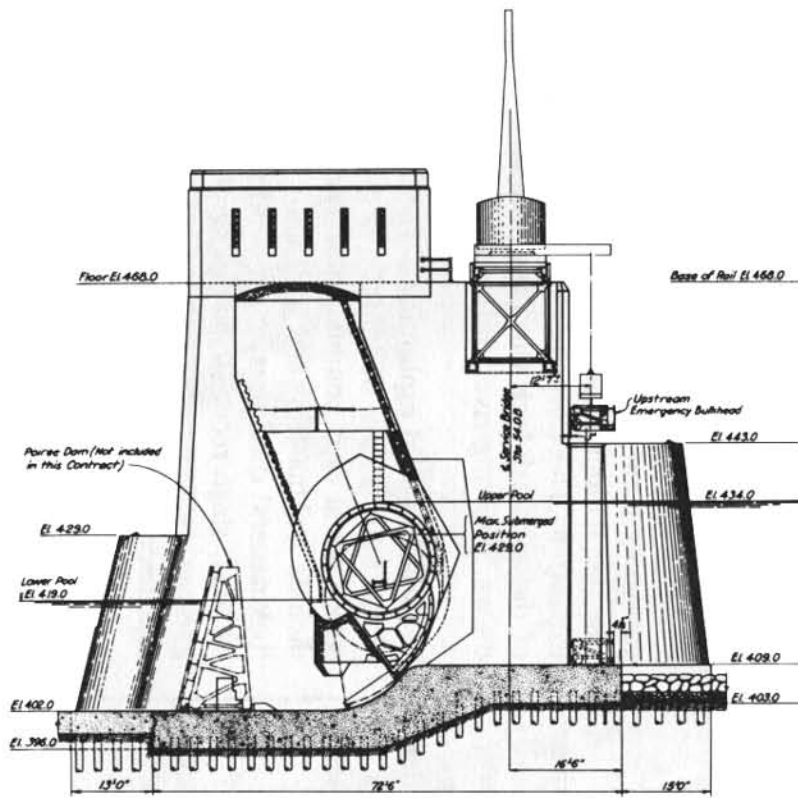
TYPICAL SECTION
