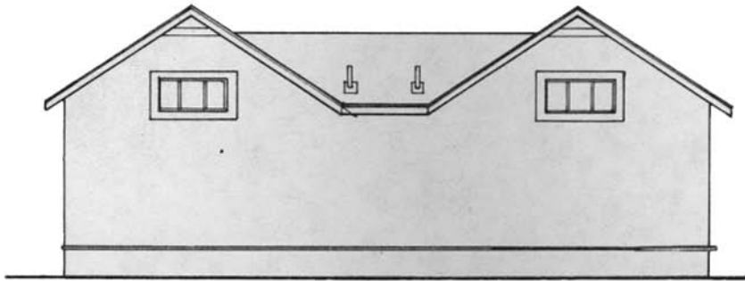
BACK ELEVATION
