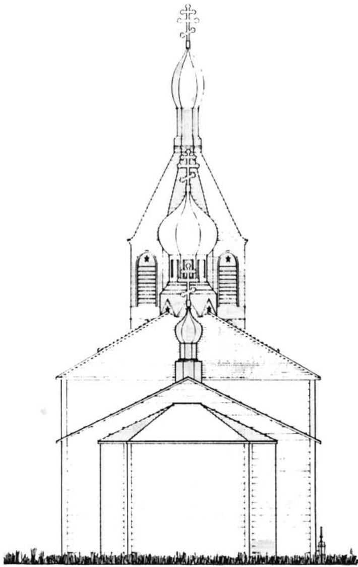
EAST ELEVATION SCALE 3/8" = 1'-0"
