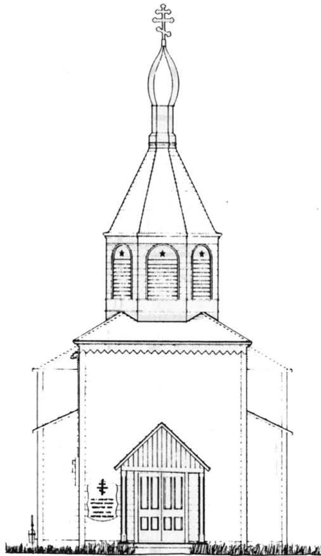
WEST ELEVATION SCALE 3/8" = 1'-0"
