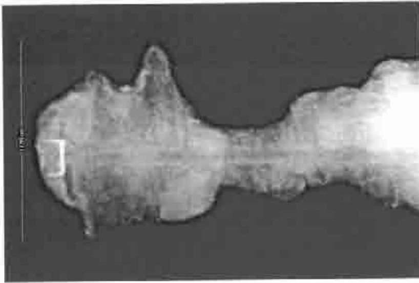
Figure 6.6. Hunhou 99-089 radiograph showing hollow mold of iron bolt with associated wood and caulking. WLCC photo.
