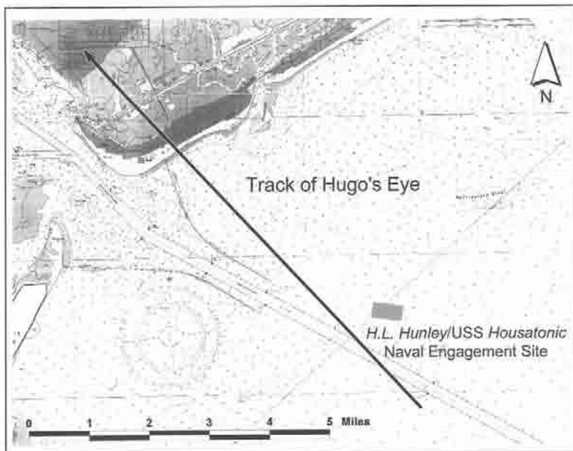
Figure 8.22. Track of Hurricane Hugo over the H.L. Hunley/USS Housatonic Naval Engagement Site.
