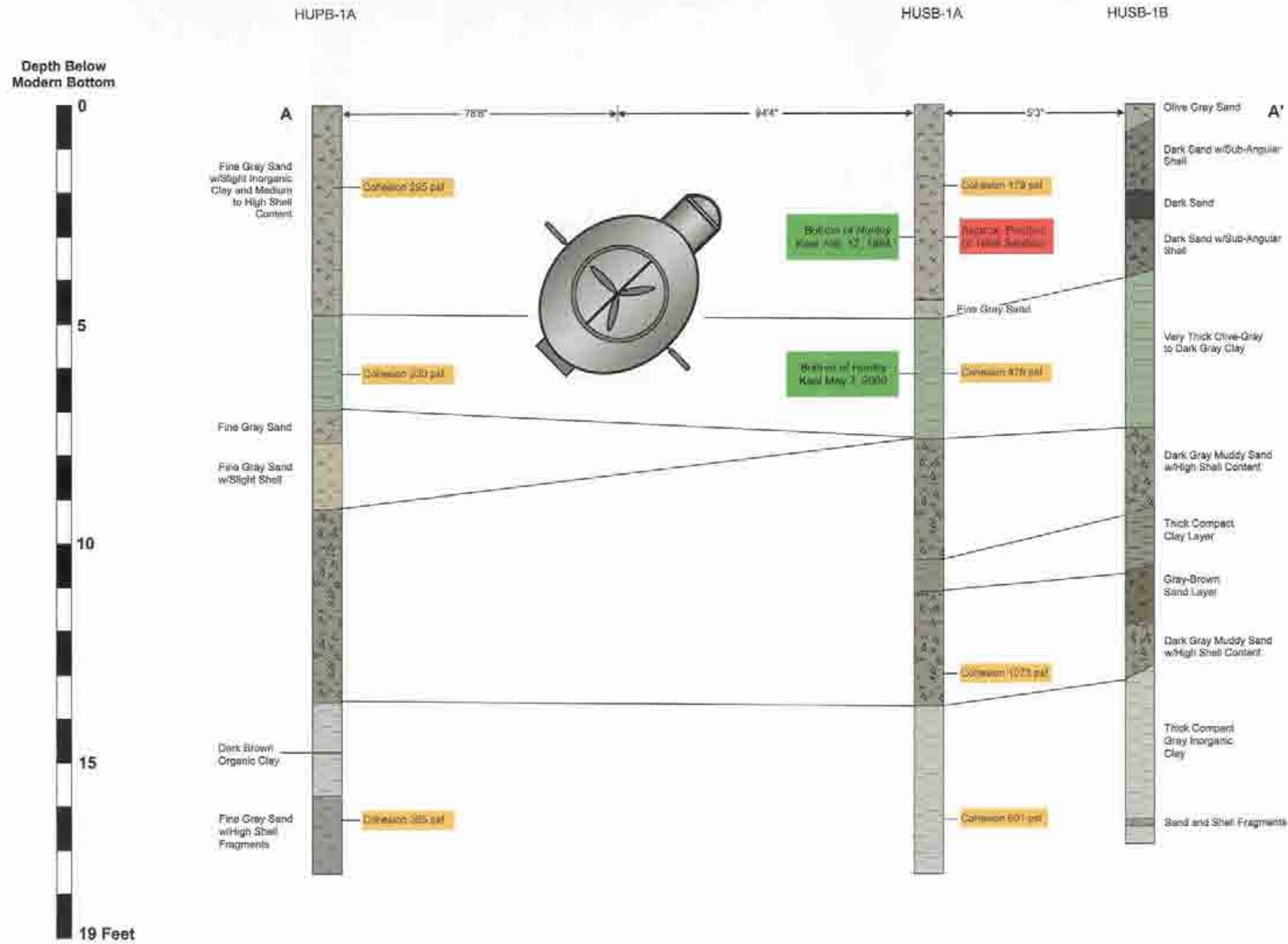
Figure 9.27. H.L. Hunley Site Stratigraphy
