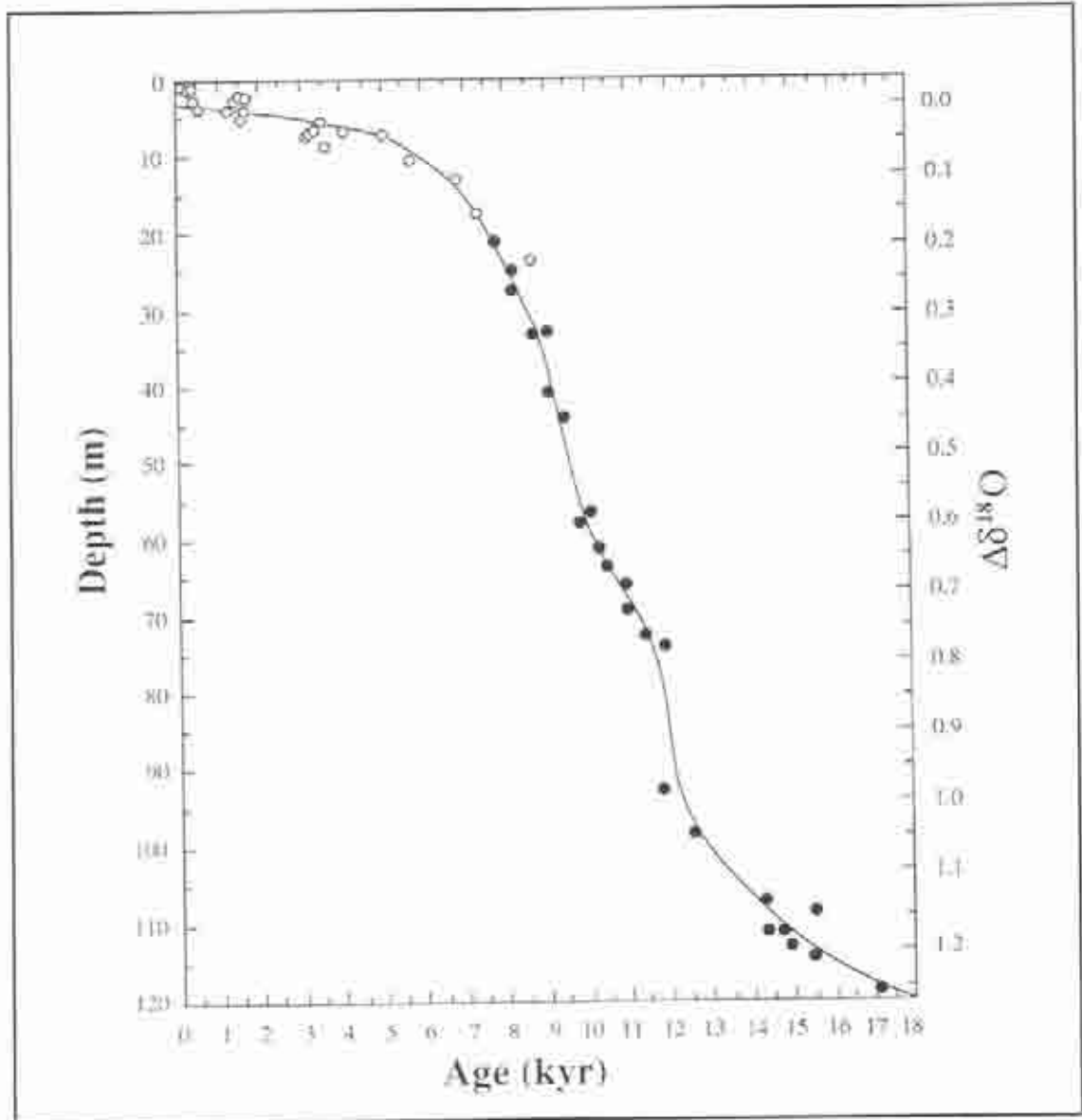
Figure 8.7. Quaternary sea level change (source R. G. Fairbanks 1989:66).
