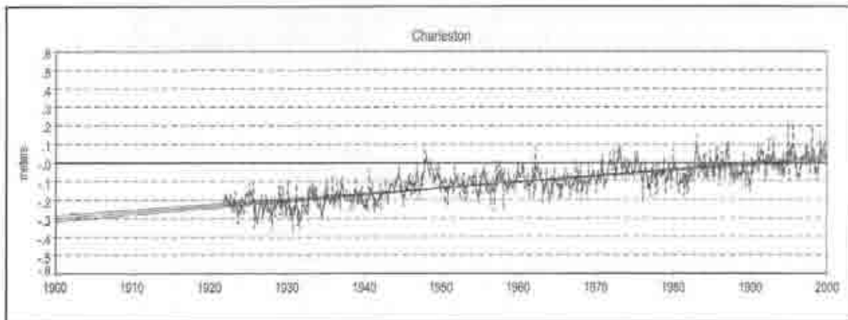
Figure 8.8. Charleston sea level trends 1921–2000 (compiled by NOAA).
