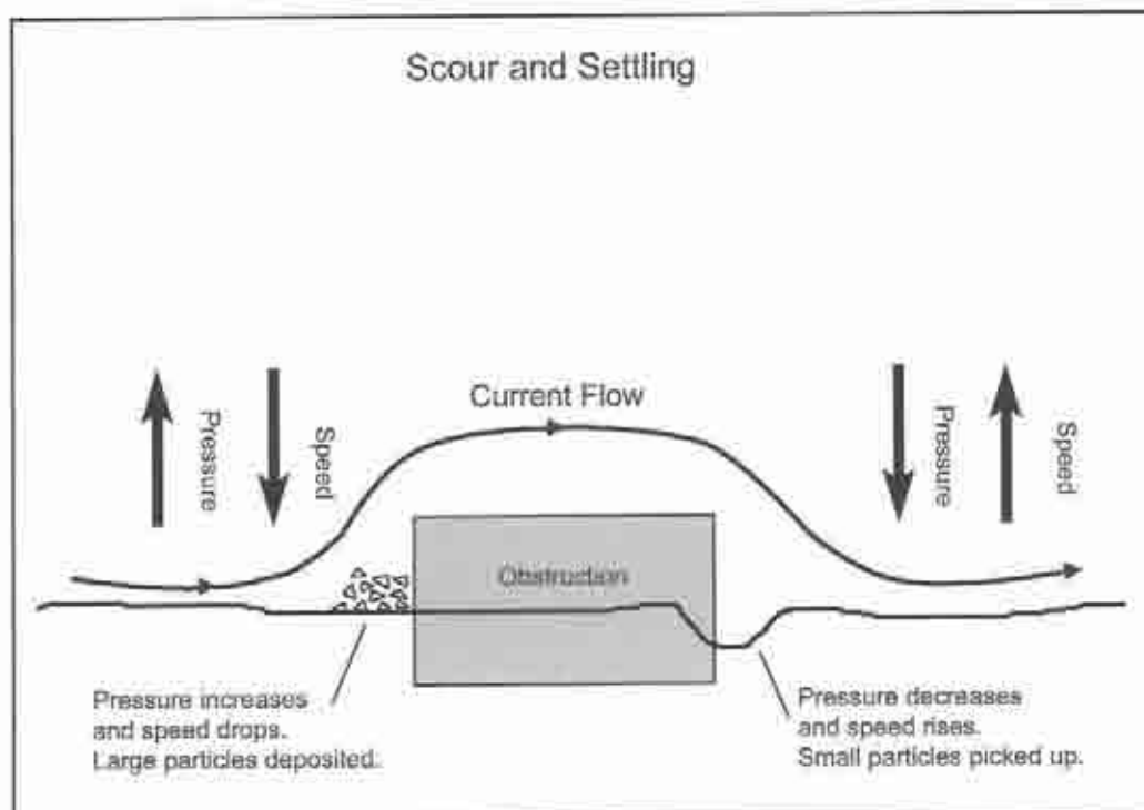
Figure 9.21. Sediment flow and deposition around an obstruction.
