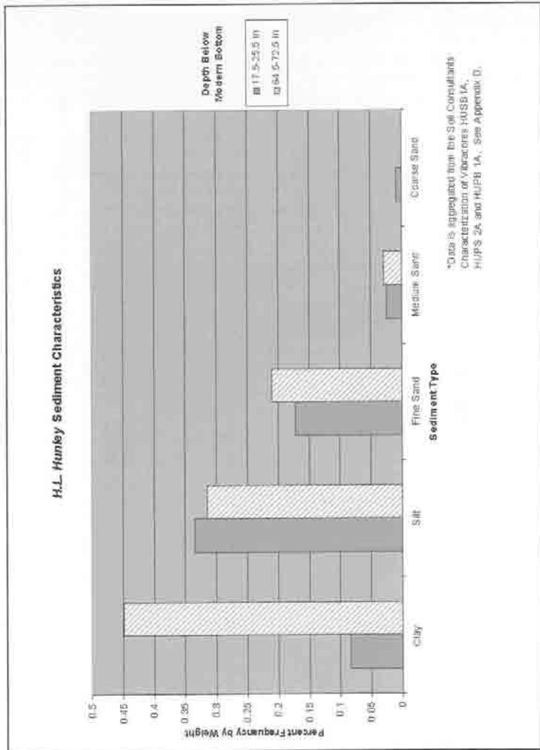
Figure 8.19. Aggregate sediment characteristics around H.L. Hunley .
