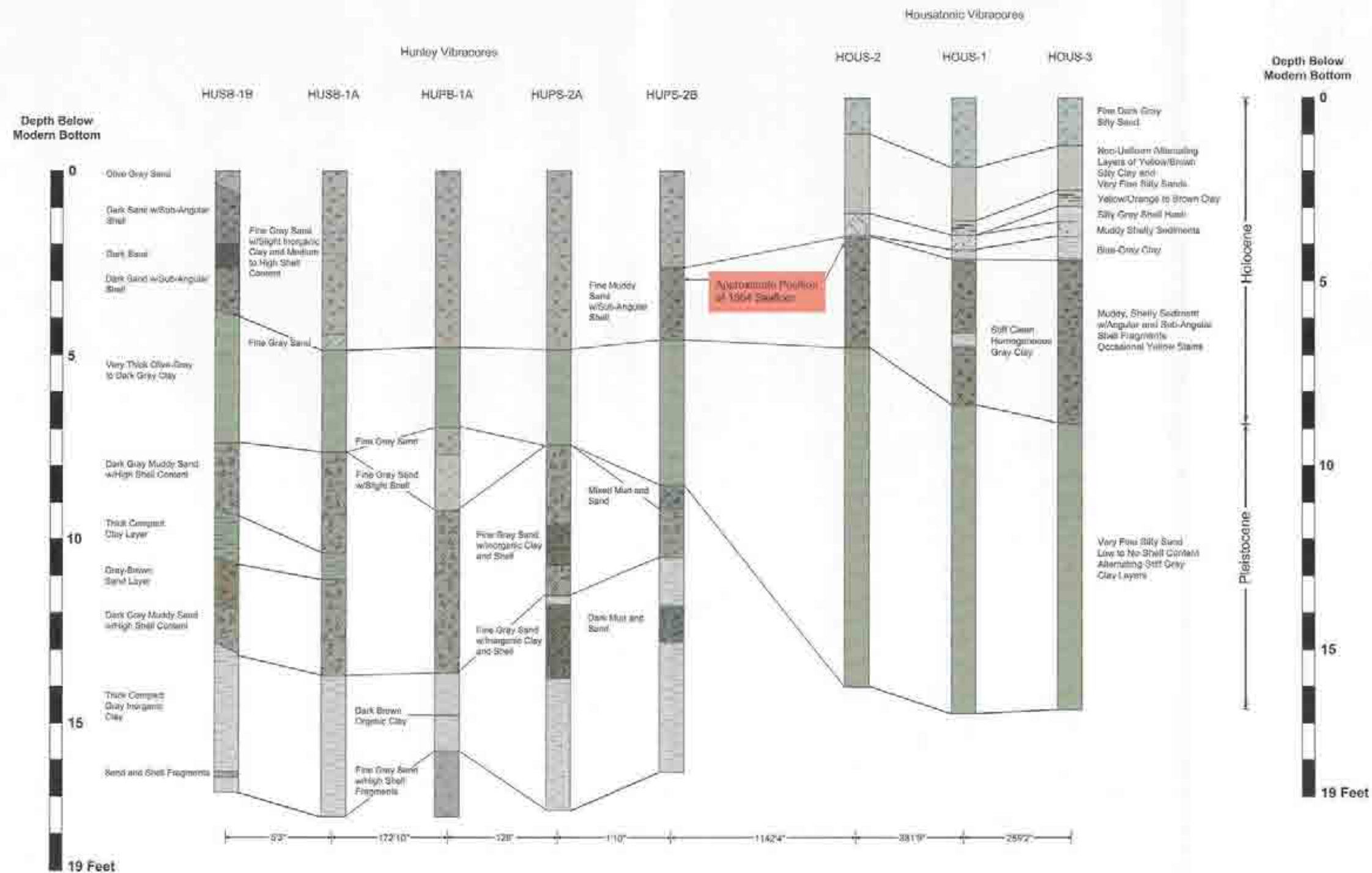
Figure 8.14. H.L. Hunley/USS Housatonic Naval Engagement Site stratigraphy.
