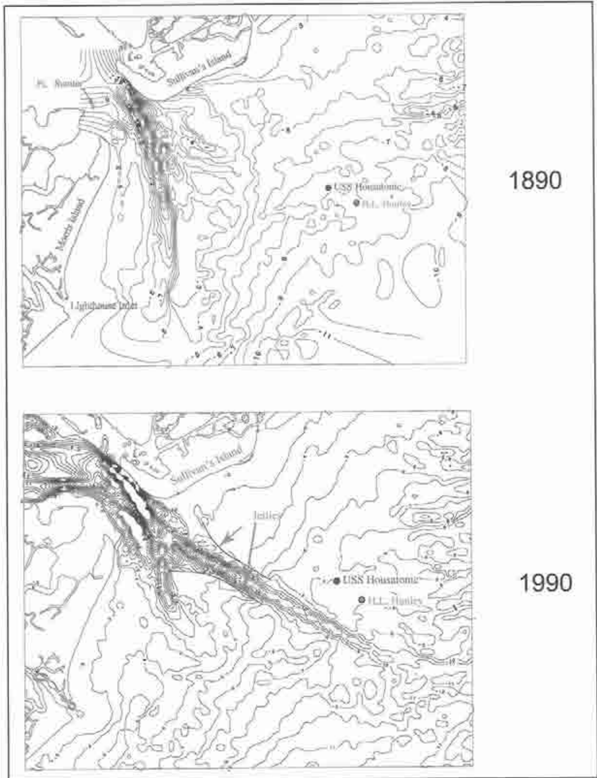
Figure 8.17. Comparative bathymetry 1890–1990 (courtesy Mark Hansen, USGS).
