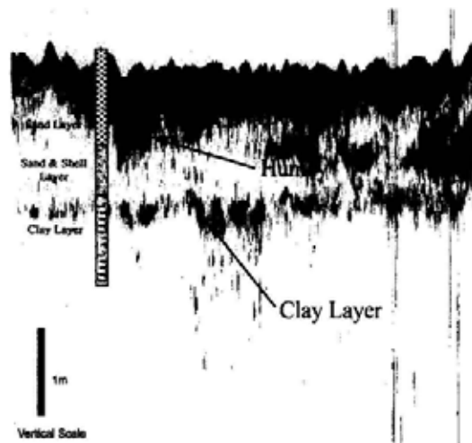
Figure 5. Example of one chirp seismic image and corresponding core log over center section of submarine.
