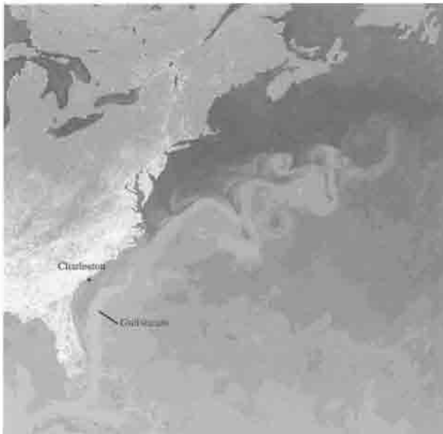
Figure 8.9. Gulf Stream (courtesy NOAA).
