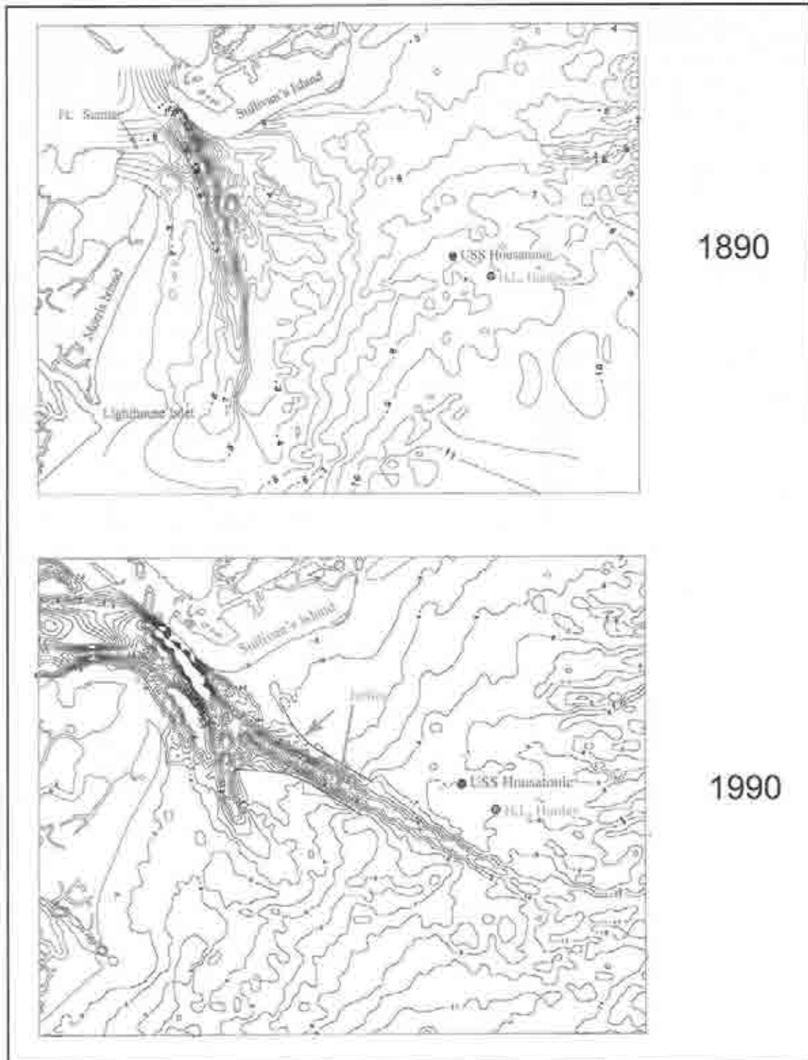
Figure 9.23. Comparative bathymetry 1890–1990. Sea level has risen on the order of 2 ft. since 1864 and depth values are not corrected (Chapter 6). All depths are in meters.
