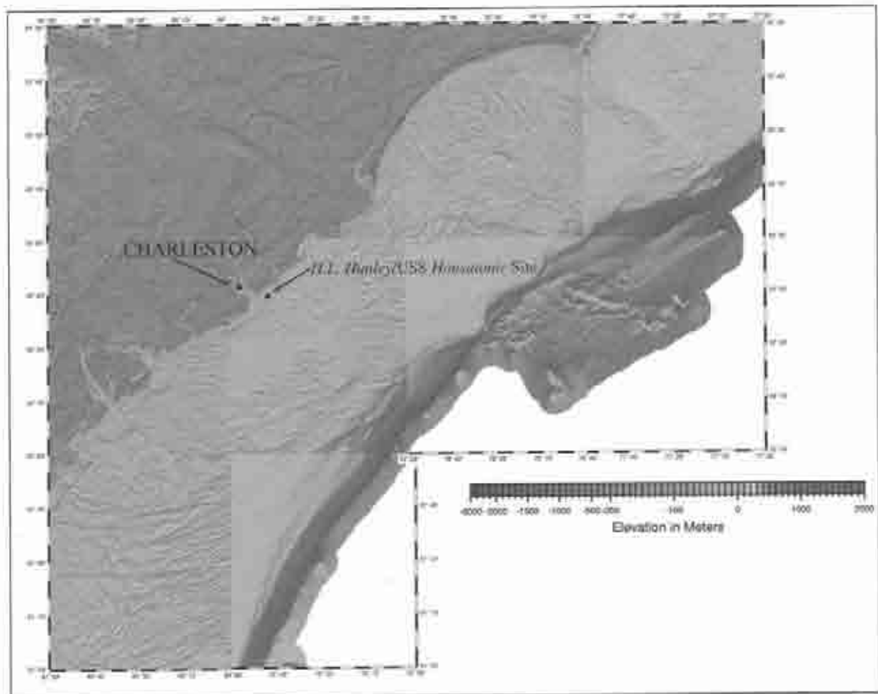
Figure 8.4. Continental Shelf of South Carolina (courtesy of National Oceanic Atmospheric Administration (NOAA)).
