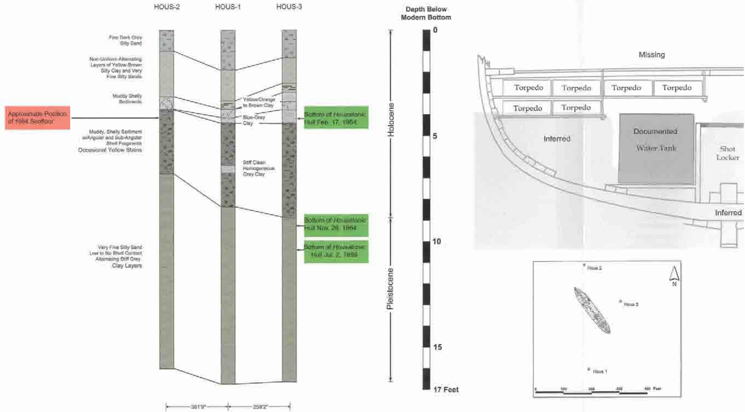
Figure 9.22. Housatonic Site Stratigraphy
