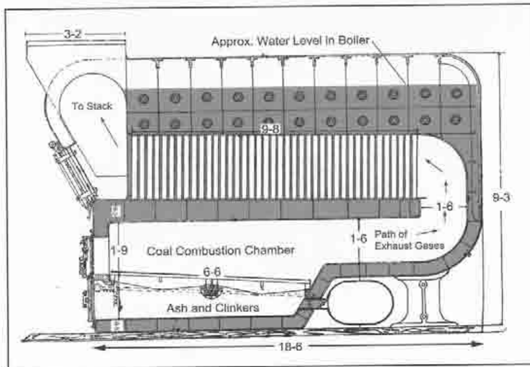
Figure 2.6. Martin vertical patent boiler. All measurements in ft.-in. (after Bennett 1896:222).
