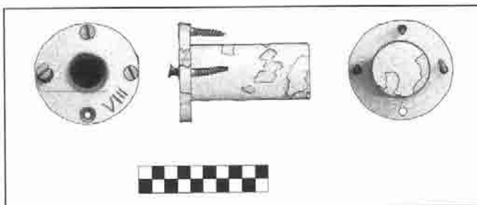
Figure 6.9. Hunhou 99-067 copper-alloy socket. NHC drawing by James Hunter.
