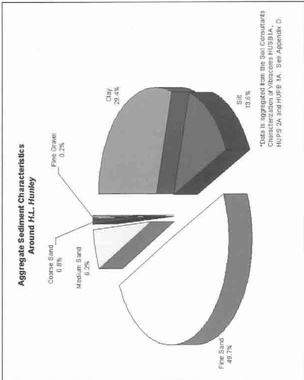
Figure 8.12. Aggregate sediment characteristics around H.L. Hunley.
