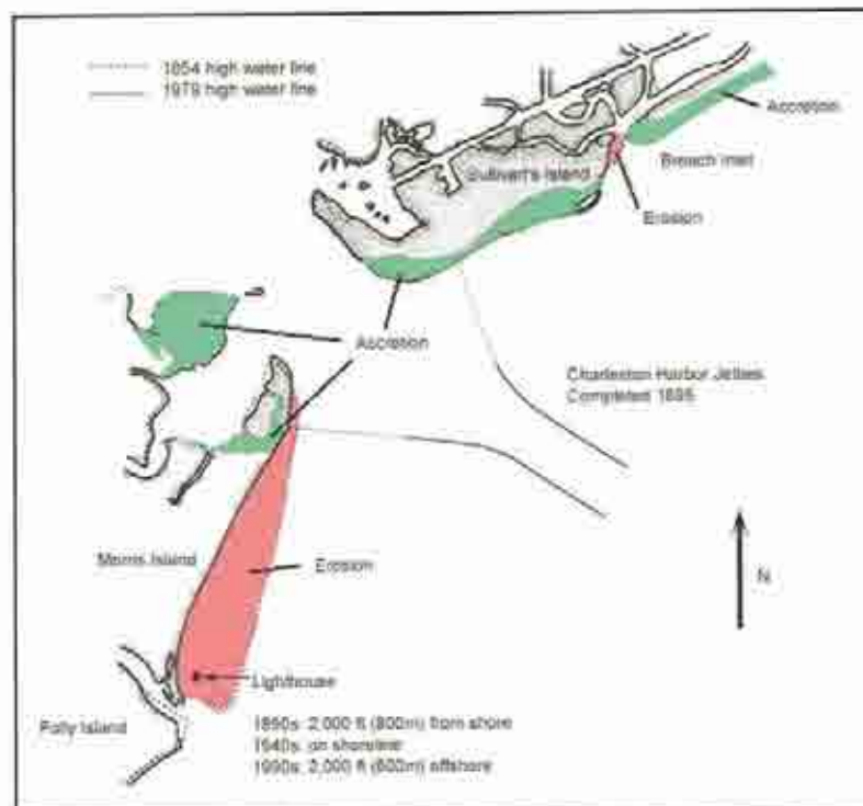
Figure 8.25. Historical changes to the Charleston coast from jetty construction (after Zarillo et al. 1985).
