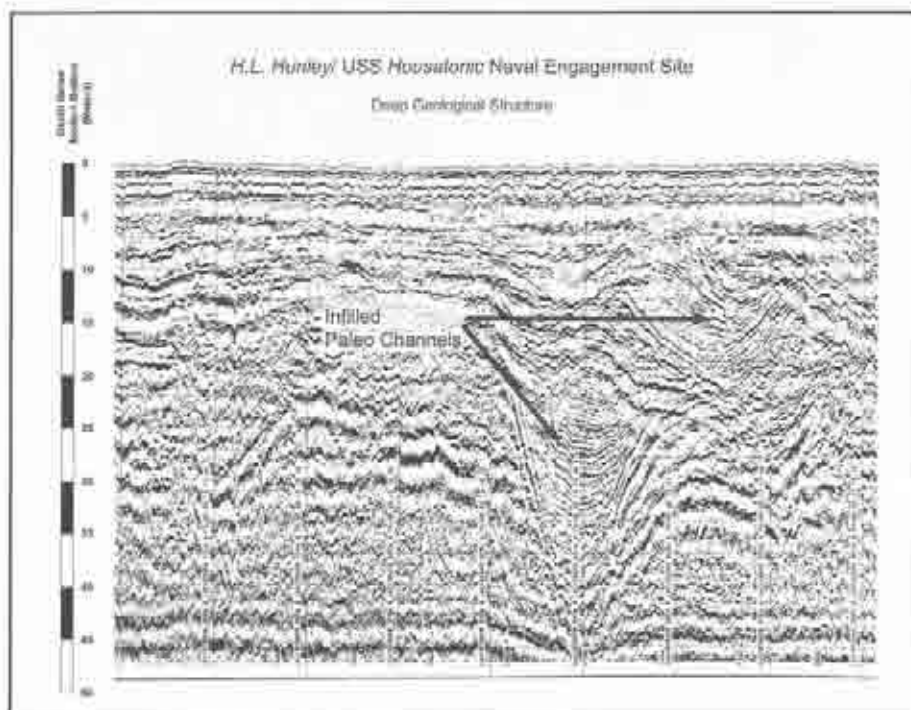
Figure 8.16. H.L. Hunley/USS Housatonic Naval Engagement Site deep geological structure.
