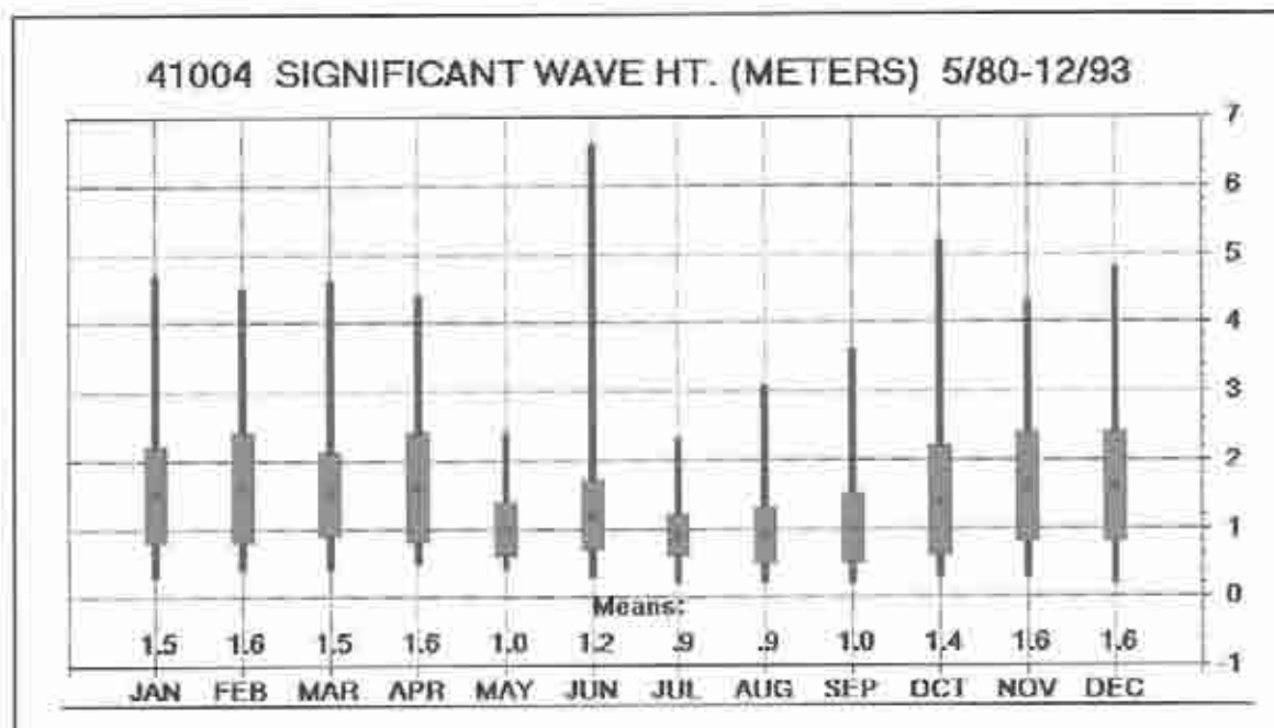
Figure 8.10. Significant wave height near the H.L. Hunley /USS Housatonic Naval Engagement Site (courtesy NOAA).
