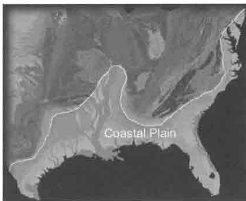
Figure 8.3. Coastal plain of the Southeastern US (courtesy of US Geological Survey (USGS)).
