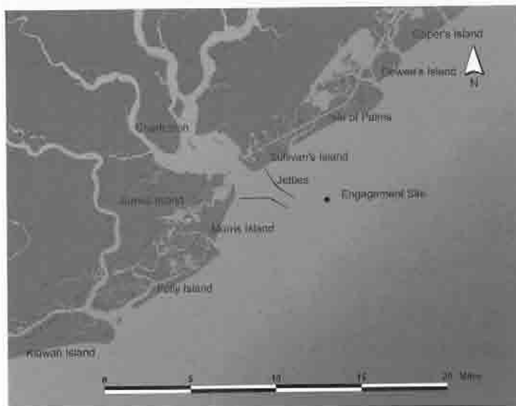
Figure 8.6. Coast of South Carolina adjacent to the H.L. Hunley /USS Housatonic Naval Engagement Site.
