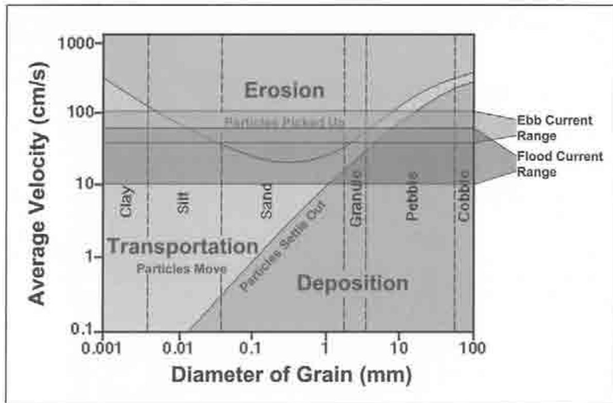
Figure 8.18. Hjulstrom diagram with ebb and flood current ranges (after Holmes 2001).
