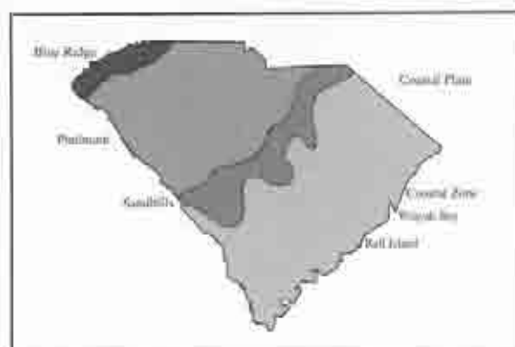
Figure 8.2. South Carolina's major physiographic zones.
