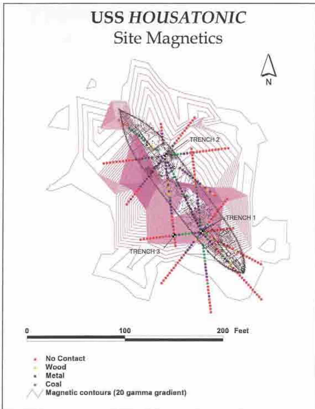
Figure 9.19. Housatonic and site magnetics.
