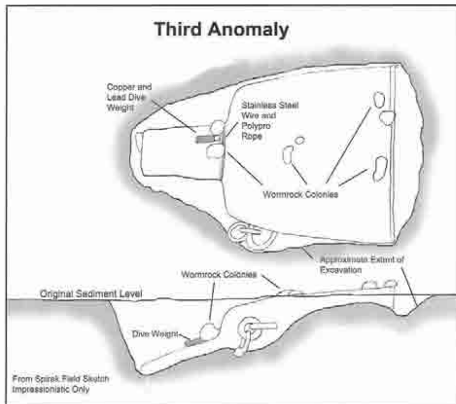
Figure 5.7. Diver's sketch of the Third Anomaly.
