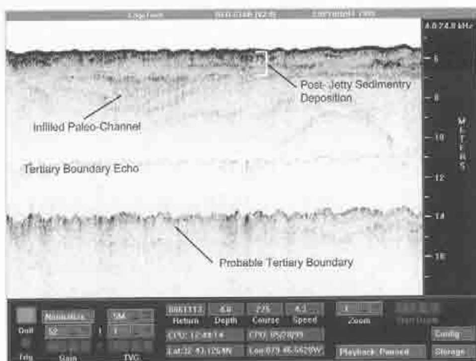
Figure 8.15. Geo-star CHIRP sub-bottom image of sediments around the H.L. Hunley/USC Housatonic Naval Engagement Site.
