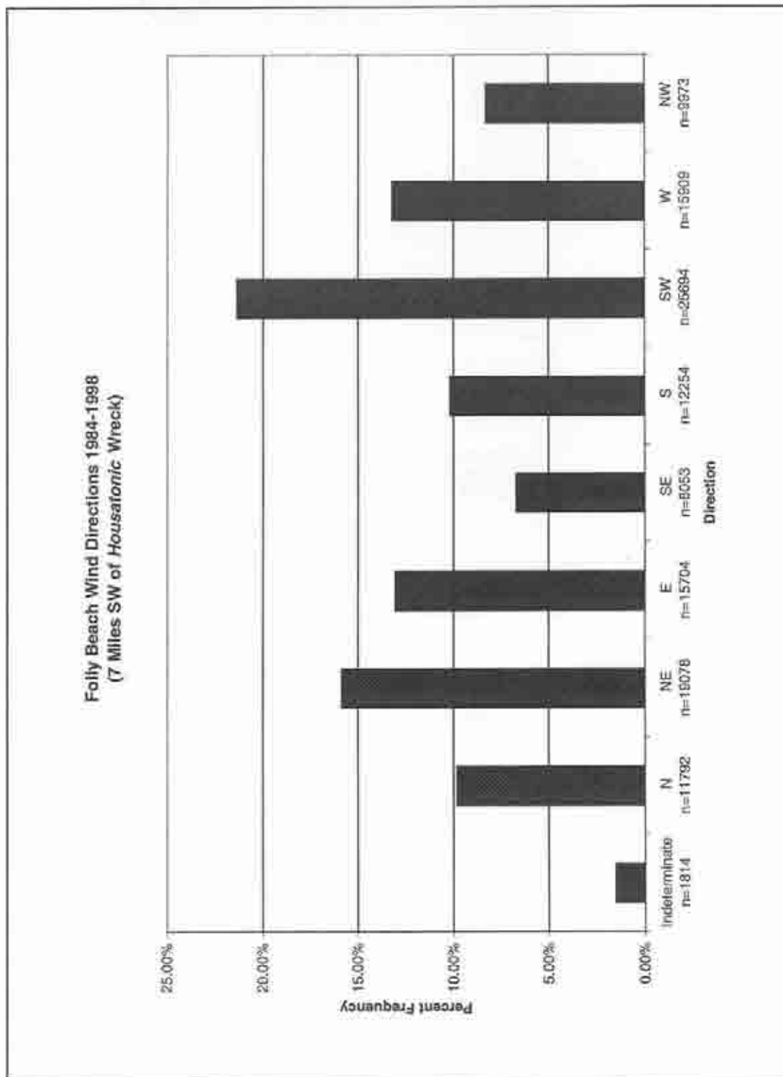
Figure 8.20. Folly Beach wind directions 1984–1998 (courtesy NOAA).
