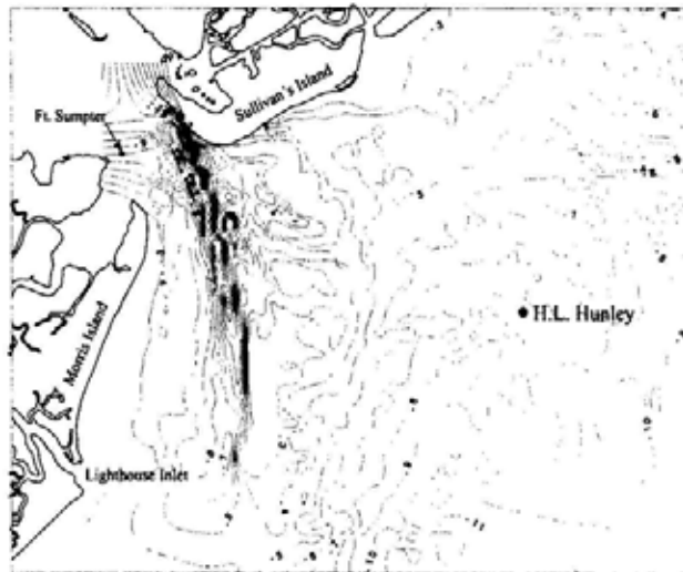
Figure 6. Bathymetric contour map of the 1880's showing location of the main ebb-channel along Morris Island and the location of the Hunley wreck site.
