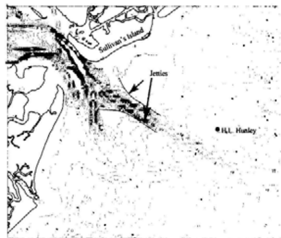
Figure 7. Location of the main ebb-channel since jetty construction and proximity to the Hunley wreck site.
