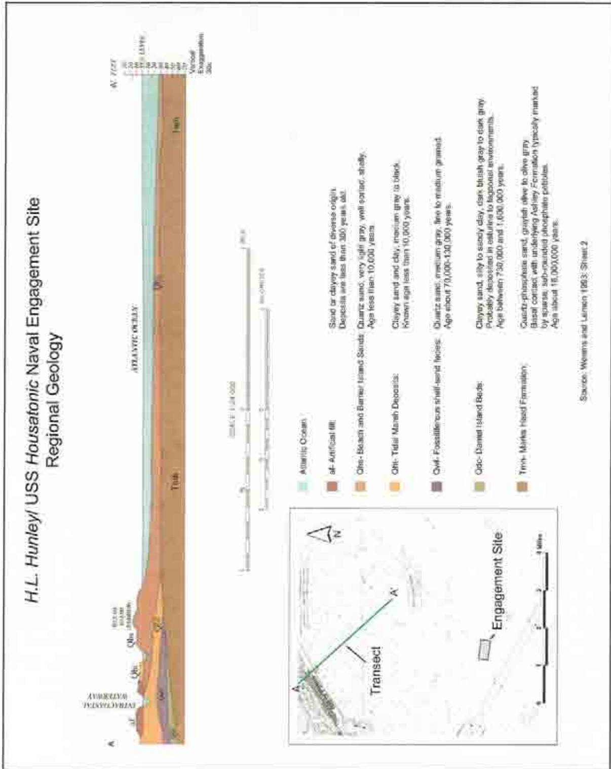
Figure 8.5. Regional geology of the H.L. Hunley/ USS Housatonic Naval Engagement Site (after Weems and Lemon 1983:Sheet 2).
