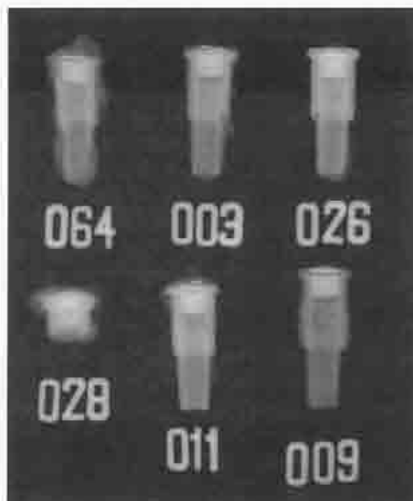
Figure 6.26. Radiograph of zinc artillery fuses from Housatonic (courtesy Navy Explosive Ordnance Disposal).
