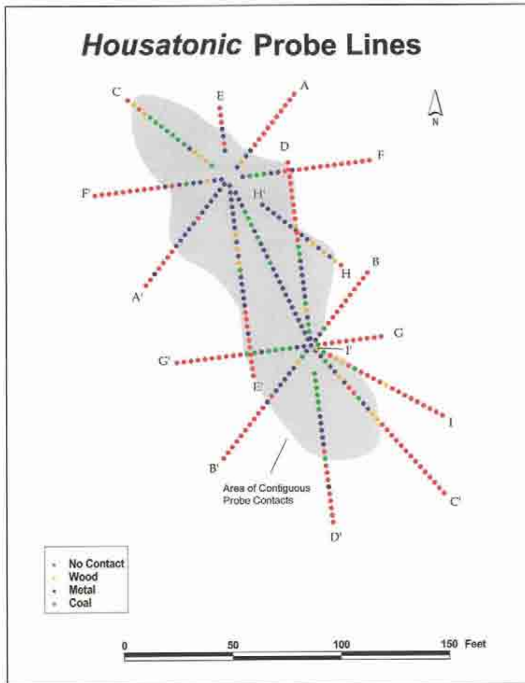
Figure 5.2. Housatonic probe lines.
