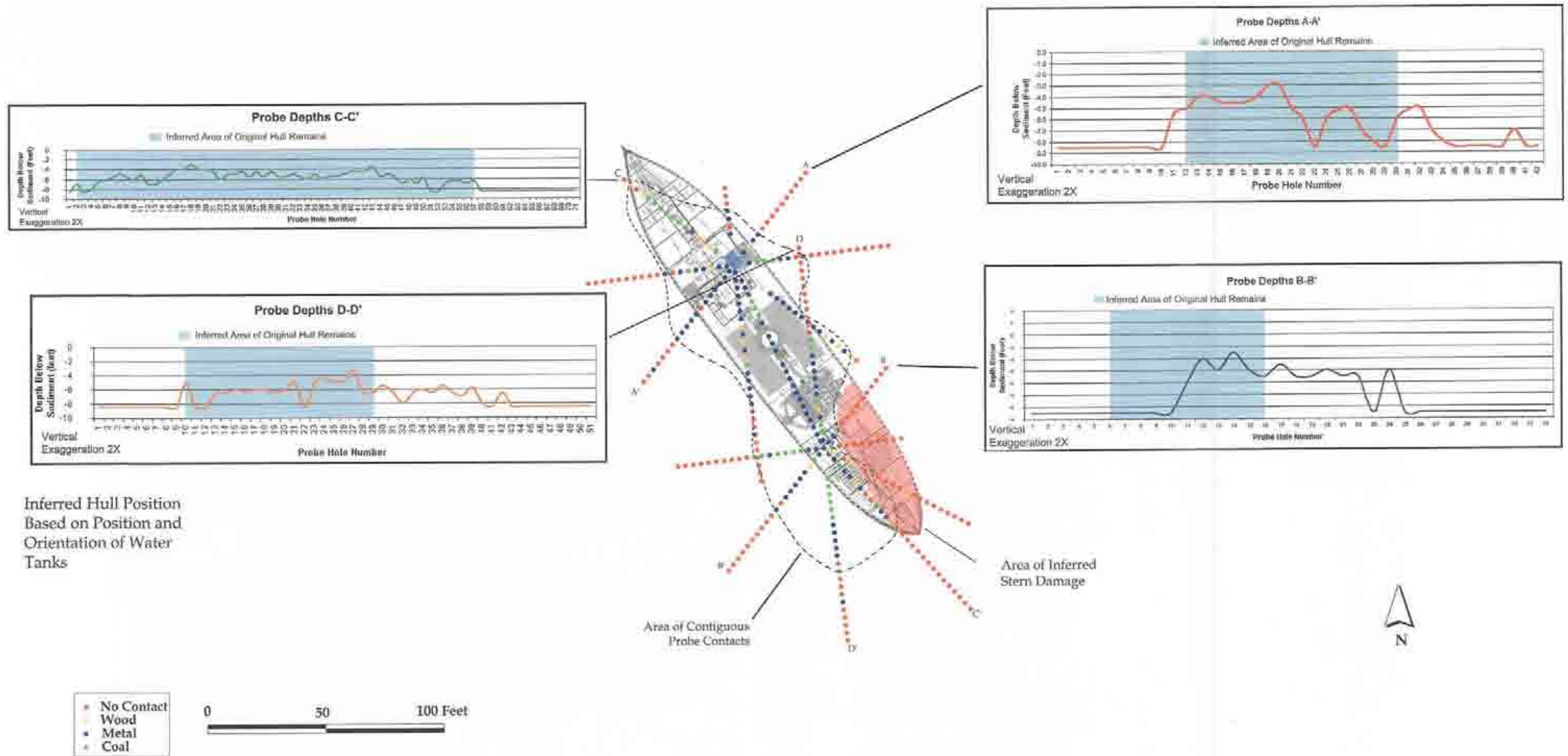
Figure 9.8. Housatonic Site 1999 Probe Lines
