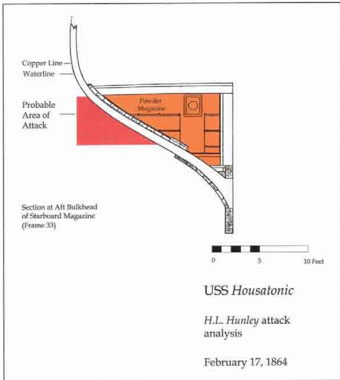
Figure 9.3. Side view of the Hunley attack.
