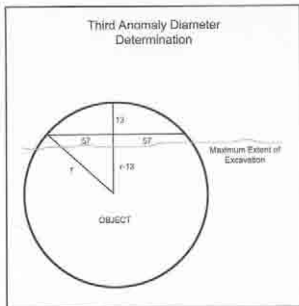
Figure 4.10. Determination of the Third Anomaly diameter.
