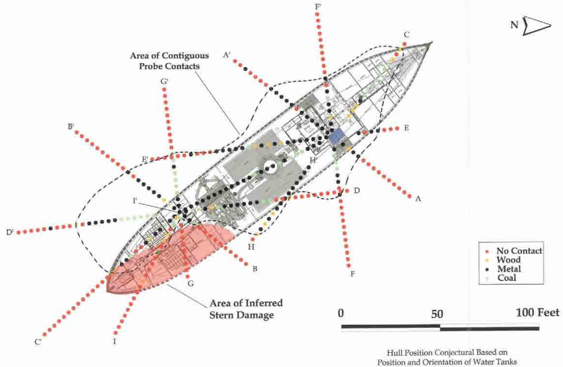
Figure 9.5. Housatonic Probe Lines and Wreck Location
