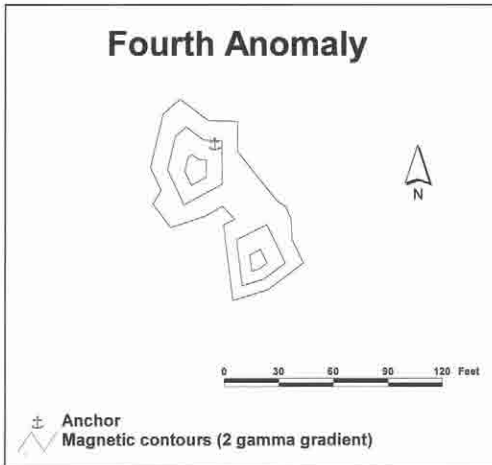
Figure 5.9. Fourth Anomaly magnetic data.
