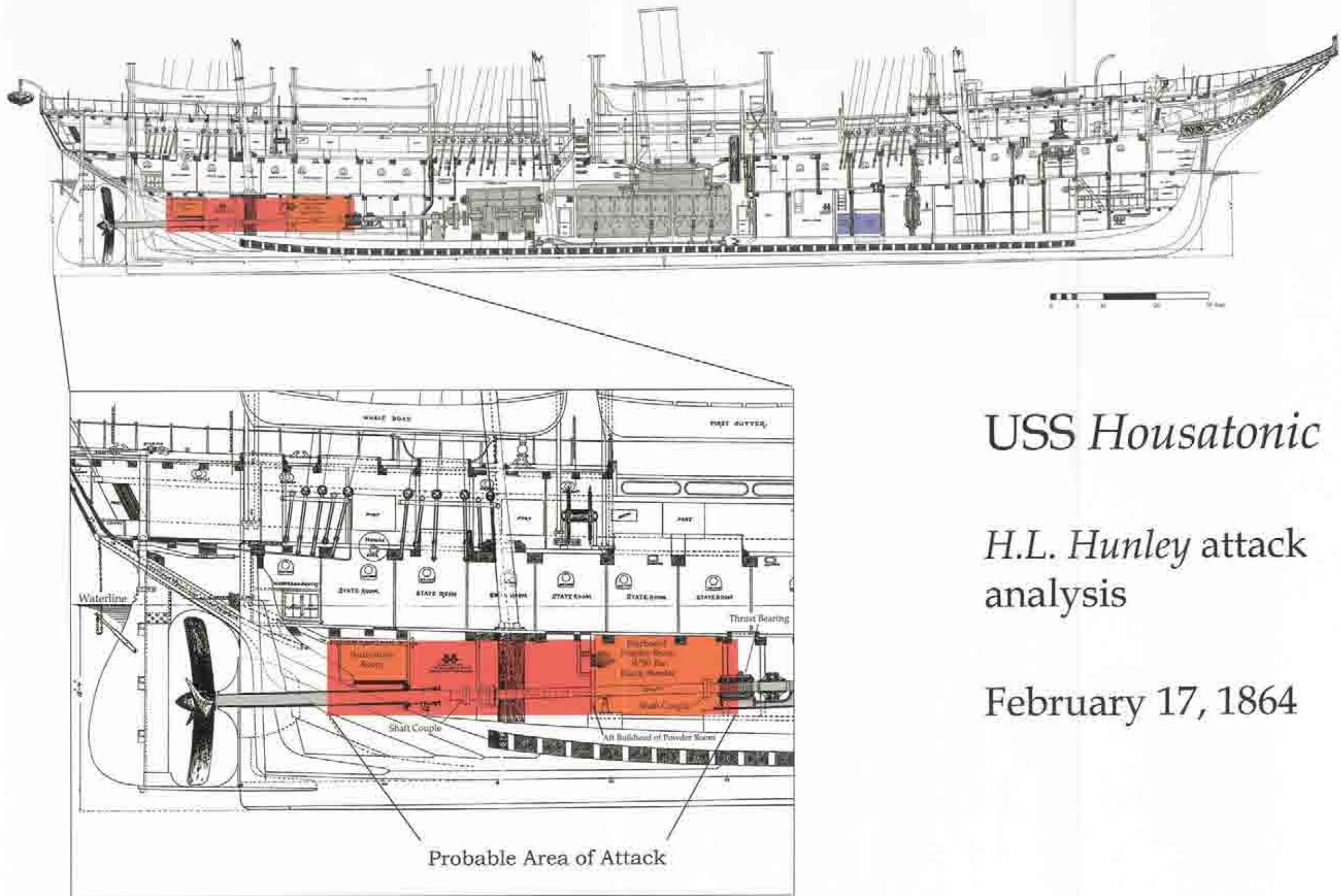
Figure 9.2. Starboard Side View of the Attack
