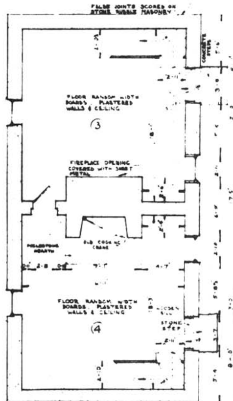
FIRST FLOOR PLAN SCALE: 1/4" = 1'-0"
