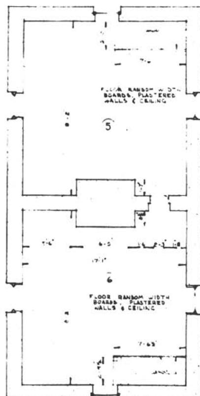
SECOND FLOOR PLAN SCALE: 1/4" = 1'-0"
