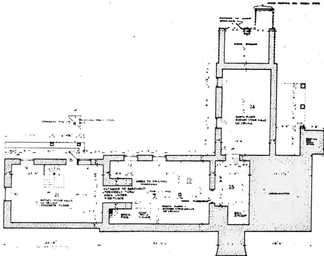
BASEMENT PLAN
