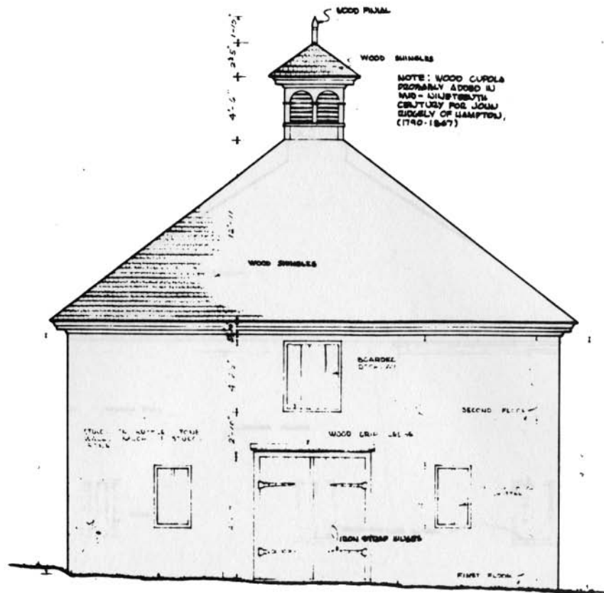
EAST ELEVATION
