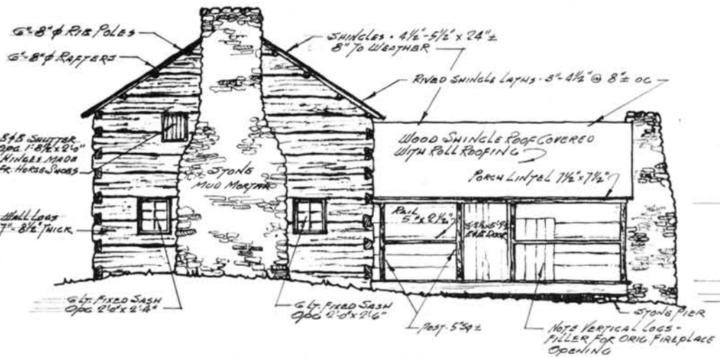
• SOUTH (FRONT) ELEVATION •
