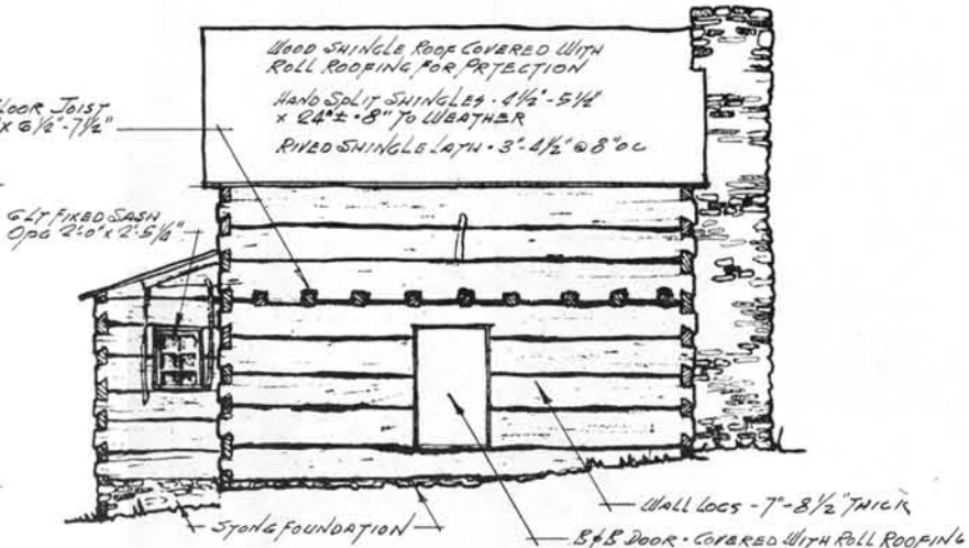
• WEST ELEVATION •
