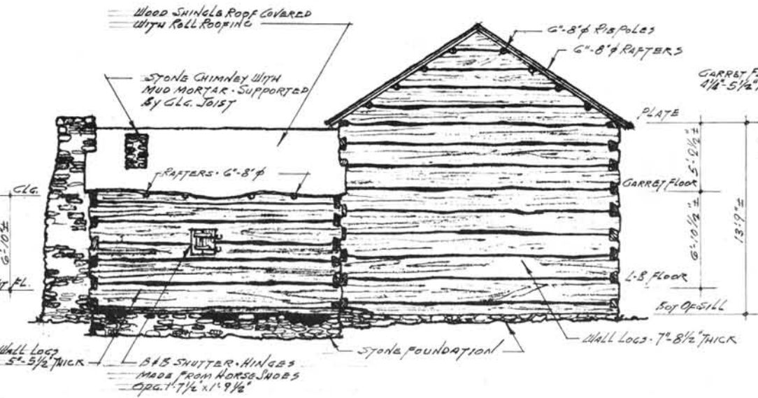
• NORTH (REAR) ELEVATION •
