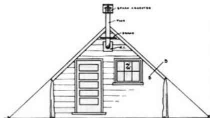
ELEVATION OF HOSPITAL & INFIRMARY BOTH ENDS SIMILAR ALSO APPLIES TO ADMINISTRATION UNIT 1/4\"/>
