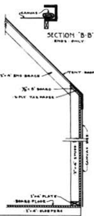
SECTION OF SIDE-WALL 3/4\"/>
