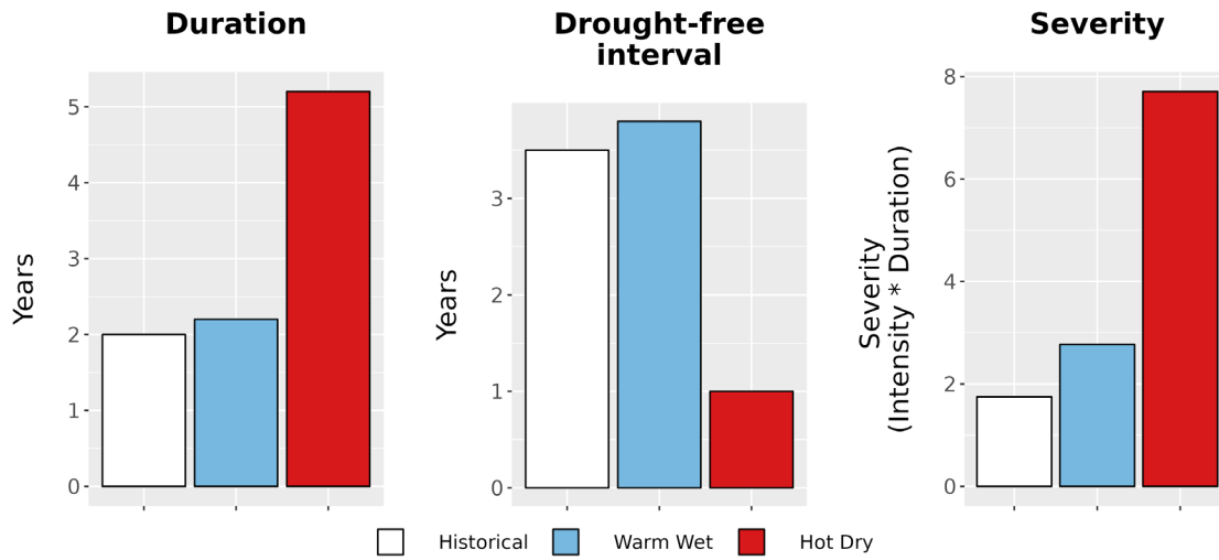
Figure 8. Drought metrics for DINO. (Left) Average drought duration (years) historically (1979-2012) and under each climate future. (Middle) Average drought return interval (years), indicating the expected amount of time between periods of drought, historically and under each climate future. (Right) Average drought severity, a measure of drought intensity multiplied by duration, historically and under each climate future.
