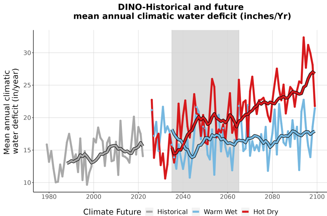
Figure 9. This line graph compares observed climatic water deficit at DINO (inches/year) (1979-2022) with projected climatic water deficit for the two climate futures over the period 2023-2099. The historical observation data is shown in gray, the Warm Wet climate future in blue, and the Hot Dry climate future in red. The smooth line running through each projection is the 10-year running average for historical observations and future projections. Gray-shaded area represents the time period that was averaged (2035-2065) to summarize future projections for the year 2050.
