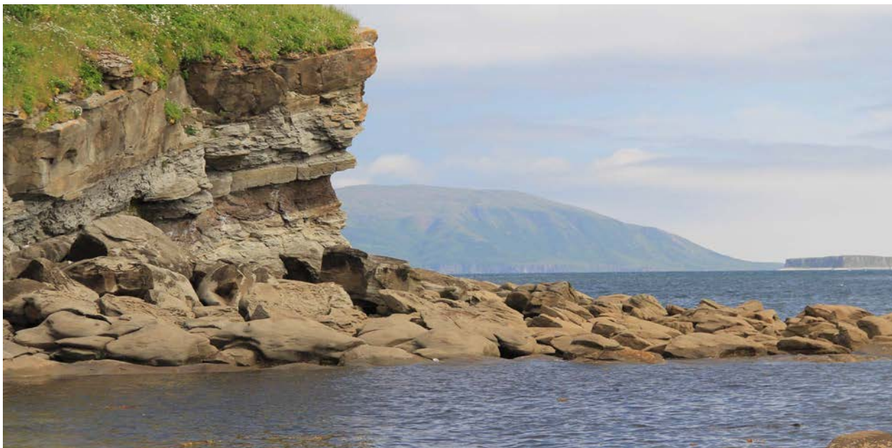
Figure 7. Coastal exposure of the Chignik Formation of Aniakchak National Monument and Preserve. These rocks represent a variety of non-marine, beach, and estuarine sedimentary environments.
