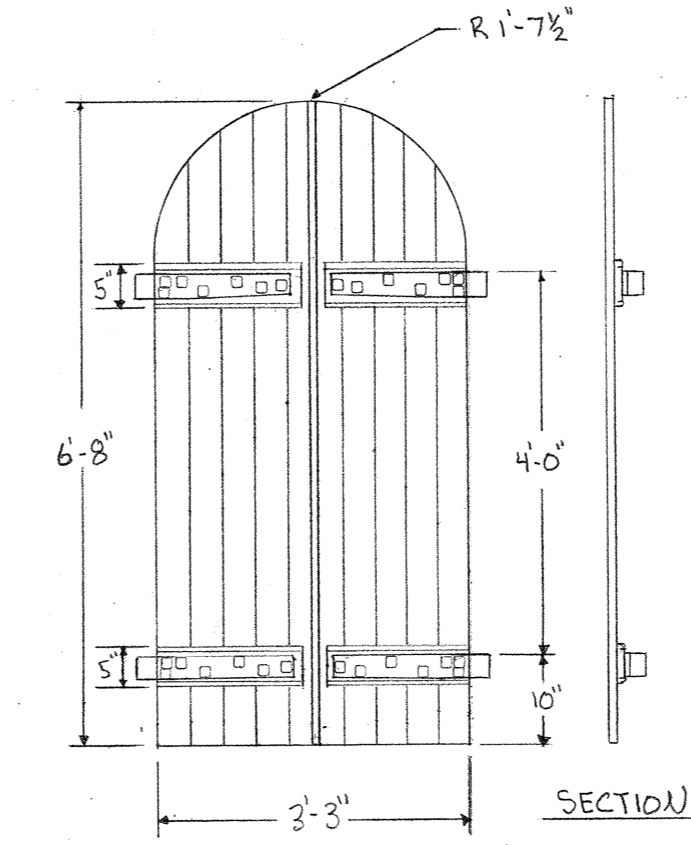
CASEMATE SHUTTERS INTERIOR ELEVATION
