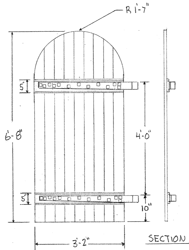
TERREPLEIN DOORS INTERIOR ELEVATION
