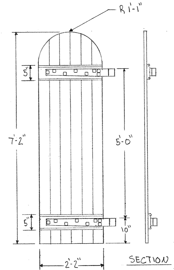
EMBRASURE SHUTTERS INTERIOR ELEVATION
