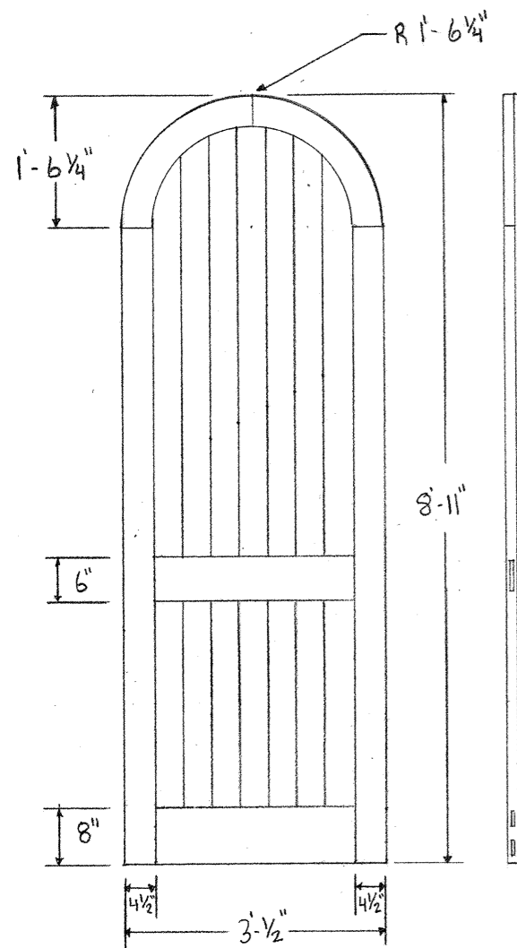
GUARDROOM DOORS INTERIOR ELEVATION
