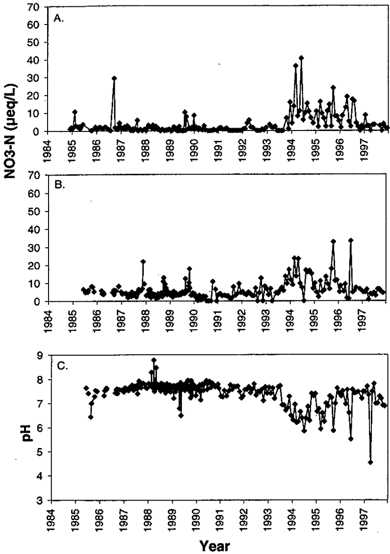
Figure 37. Concentrations of NO 3 -N in (A) precipitation falling near the West Twin Creek watershed and (B) in the stream in the watershed, 1984–1997. Stream pH is also shown (C).
