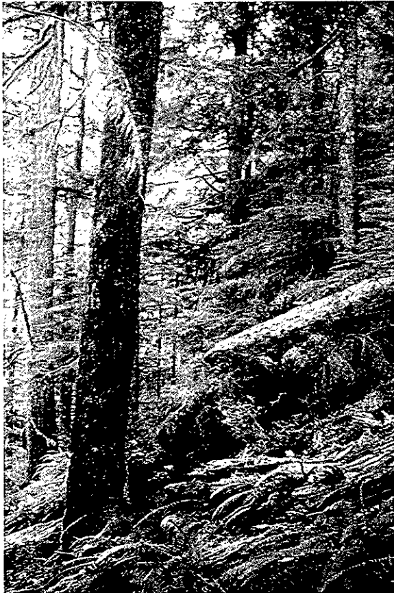
Figure 9. Permanent sampling plot 2 in the lower West Twin Creek watershed.
