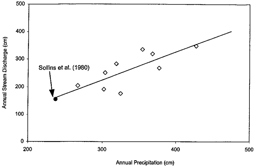
Figure 23. Annual stream discharge at the West Twin Creek weir and precipitation at the West Twin Creek from Water Year 85–86 to 93–94.
