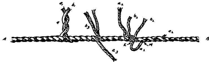
FIG. 22 LONG SPLICE (2)
