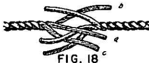
FIG. 18 SHORT SPLICE (1)
