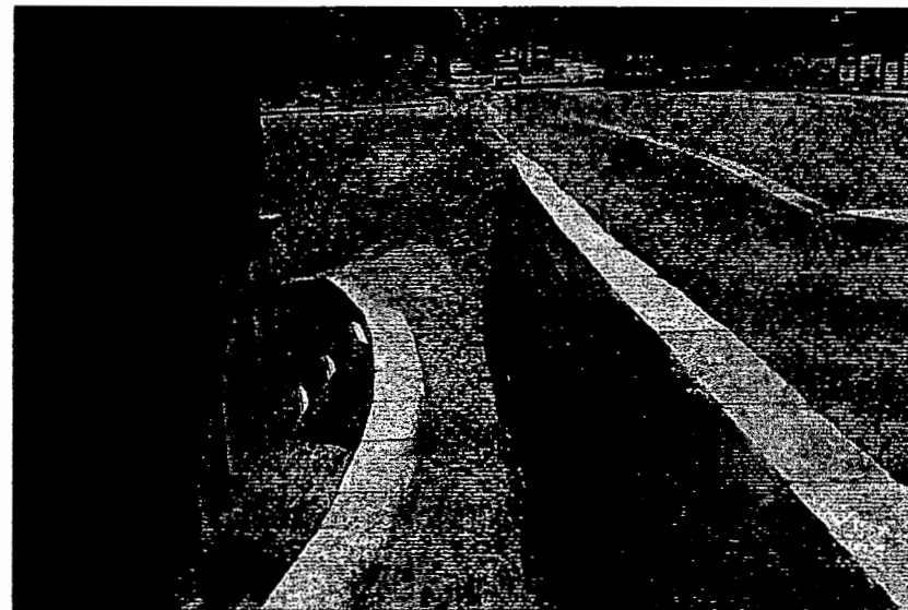
Photograph 90. Cut-stone masonry retaining wall at corner of Mule Barn. (JMA, 2001)
