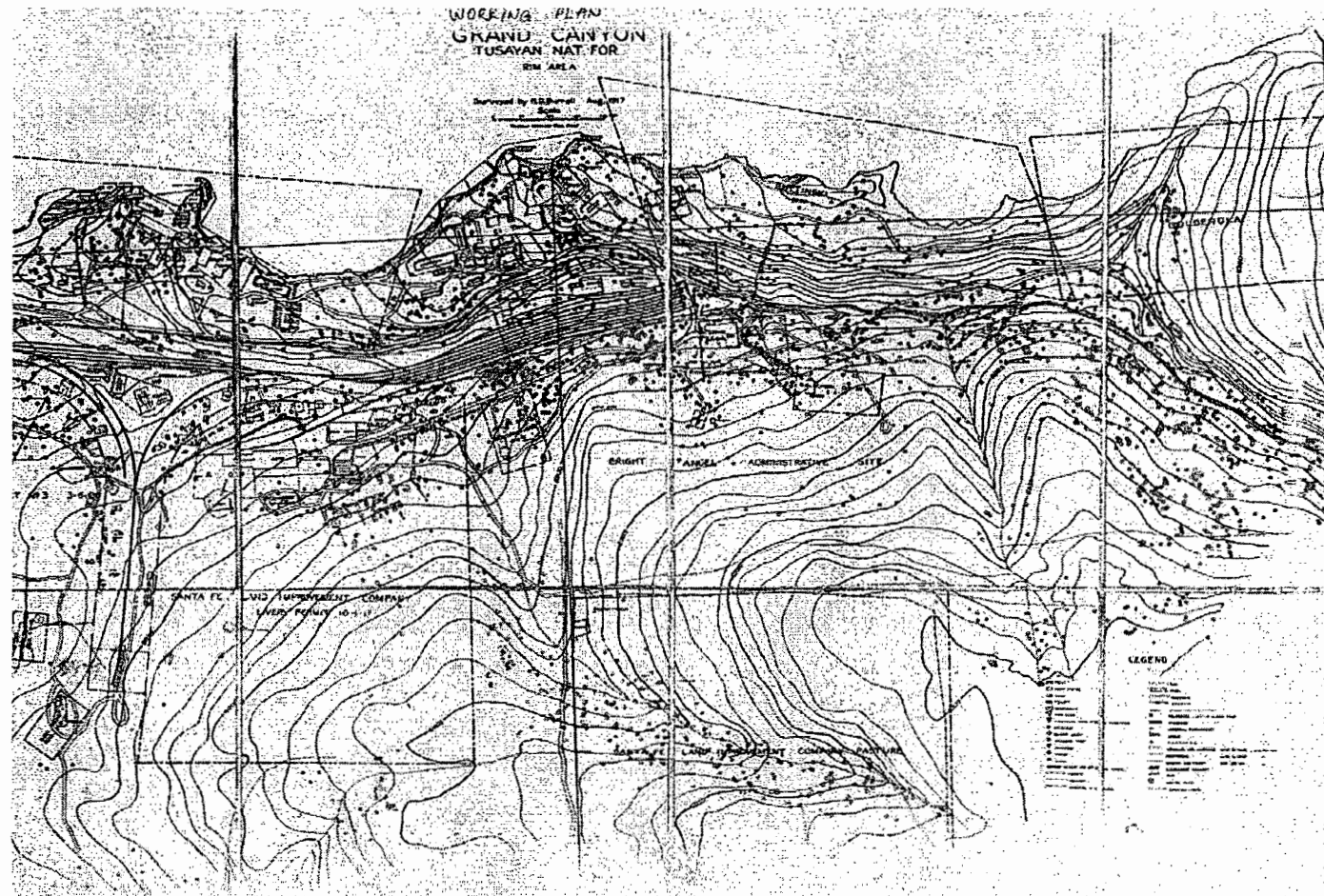
Figure 14. "Working Plan Map Grand Canyon, Tusayan National Forest, Rim Area," Surveyed by H.D. Burrall (U.S. Forest Service), August 1917. This map was the first topographical survey prepared of the Grand Canyon Village area. It depicts existing conditions and special use permits granted to various entities. (Grand Canyon Museum Collection Catalog #28344-G)
