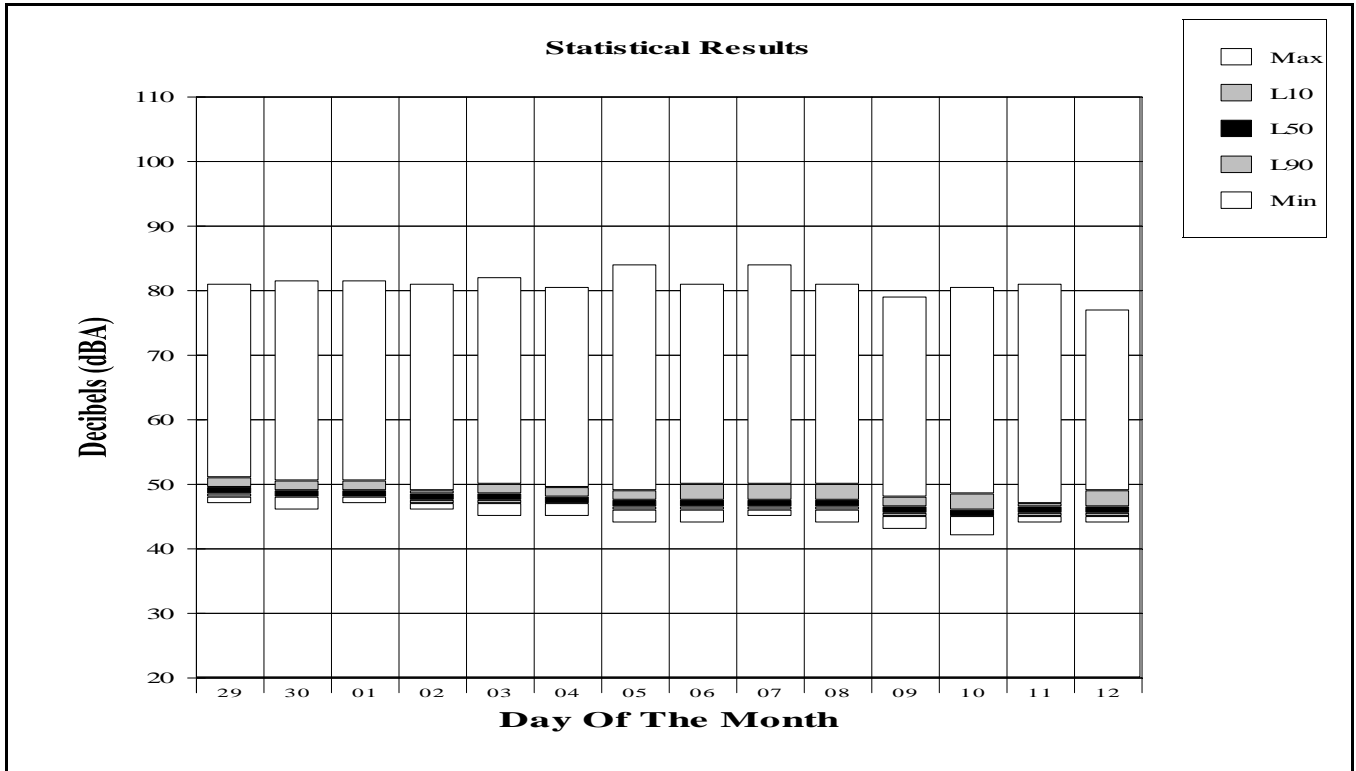
Figure 4-3 Site Specific Ambient Noise Measurement Results Jackson Hole Airport 2009 Annual Report Site: Moose
