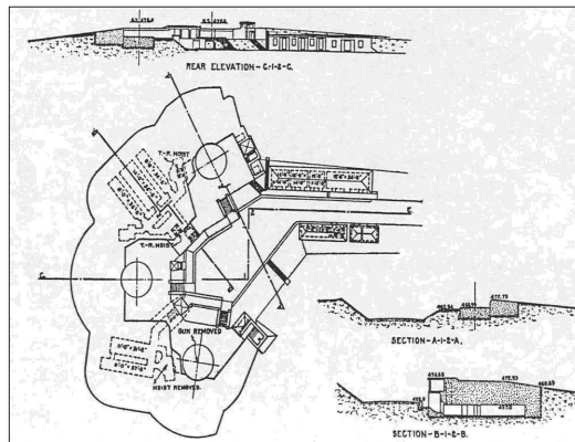
BS5 Diagram of Battery Spencer circa 1919 from "Report of Completed Works--Seacoast Fortifications."
