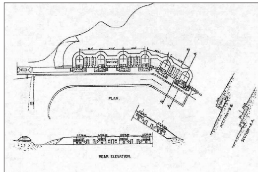
BS4 Diagram of Battery George Yates circa 1919 from "Report of Completed Work--Seacoast Fortifications."
